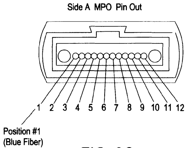
FIG. 2C METHOD B POLARITY
