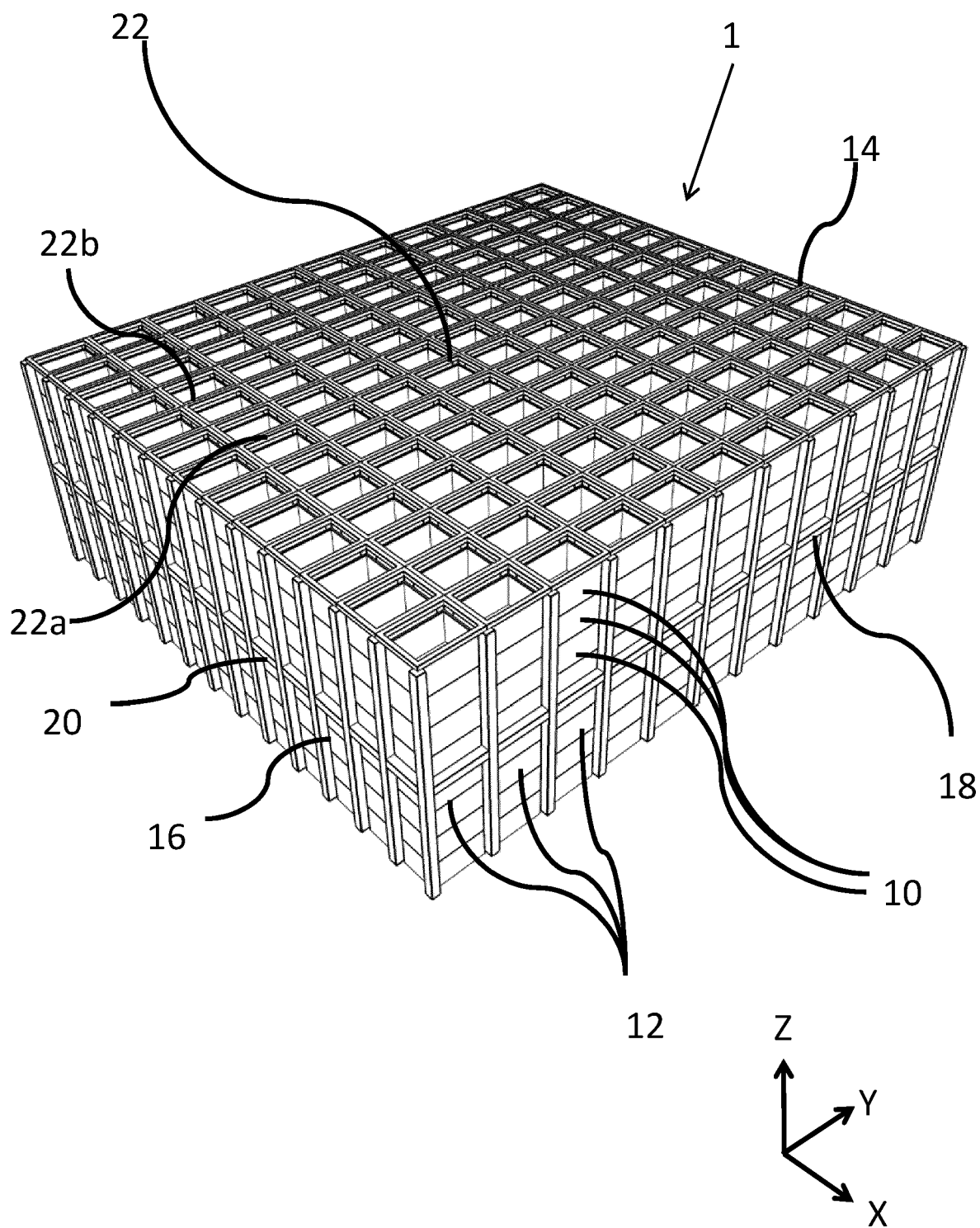
Figure 13 (PRIOR ART)
