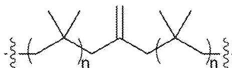
[Formula e-1]
