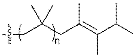
[Formula e-1]
