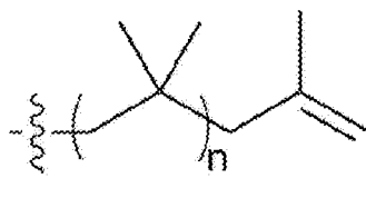
[Formula d-1]
