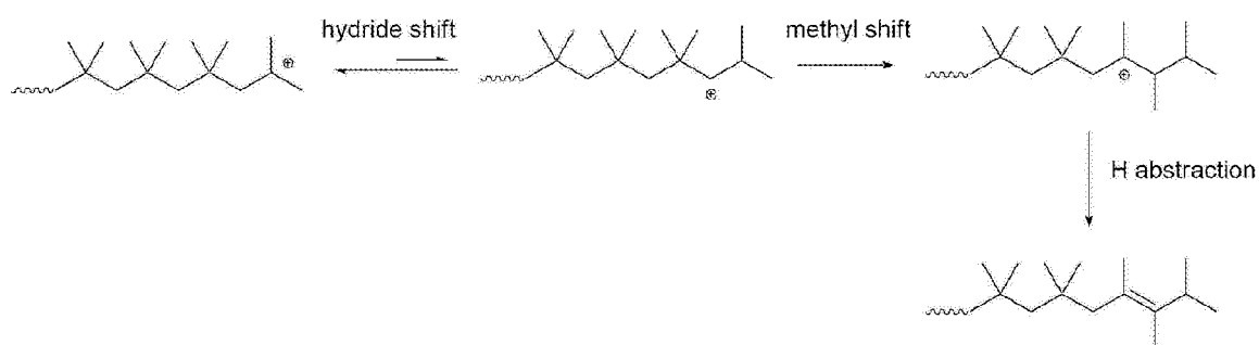
[Reaction 3]
