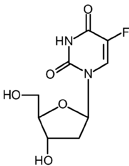
5-FdUrd
