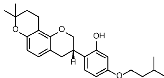
<Compound 8b>
