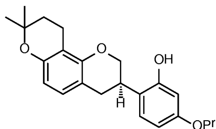
<Compound 2a>
