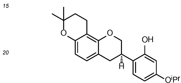
<Compound 3a>
