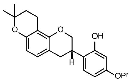
<Compound 2b>
