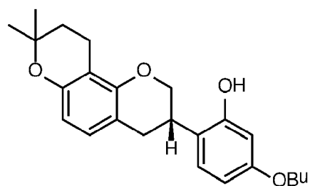
<Compound 4b>
