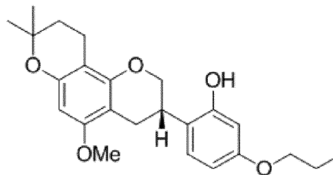
&lt;Compound 12b&gt;
