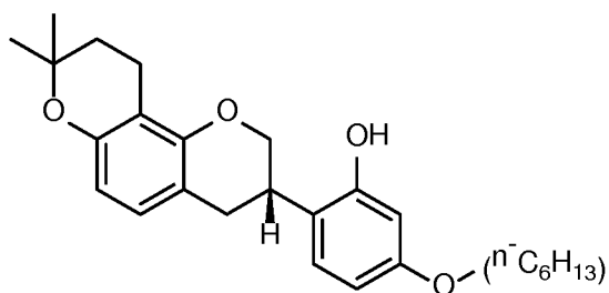
<Compound 7b>
