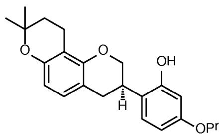
<Compound 2a>
