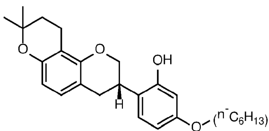
<Compound 7b>
