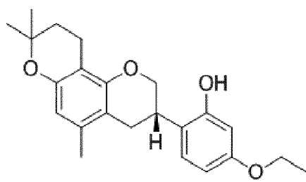
<Compound 9b>
