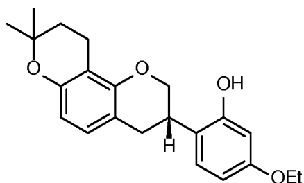
&lt;Compound 1b&gt;
