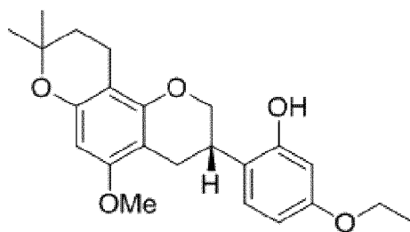
<Compound 11b>
