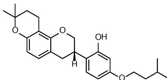
<Compound 8b>
