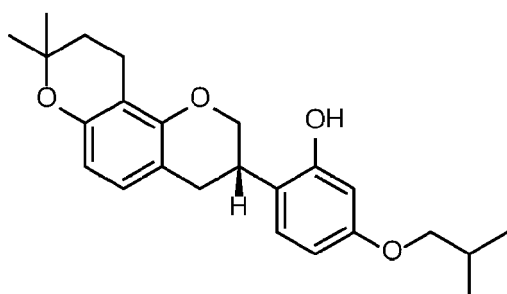
<Compound 5b>
