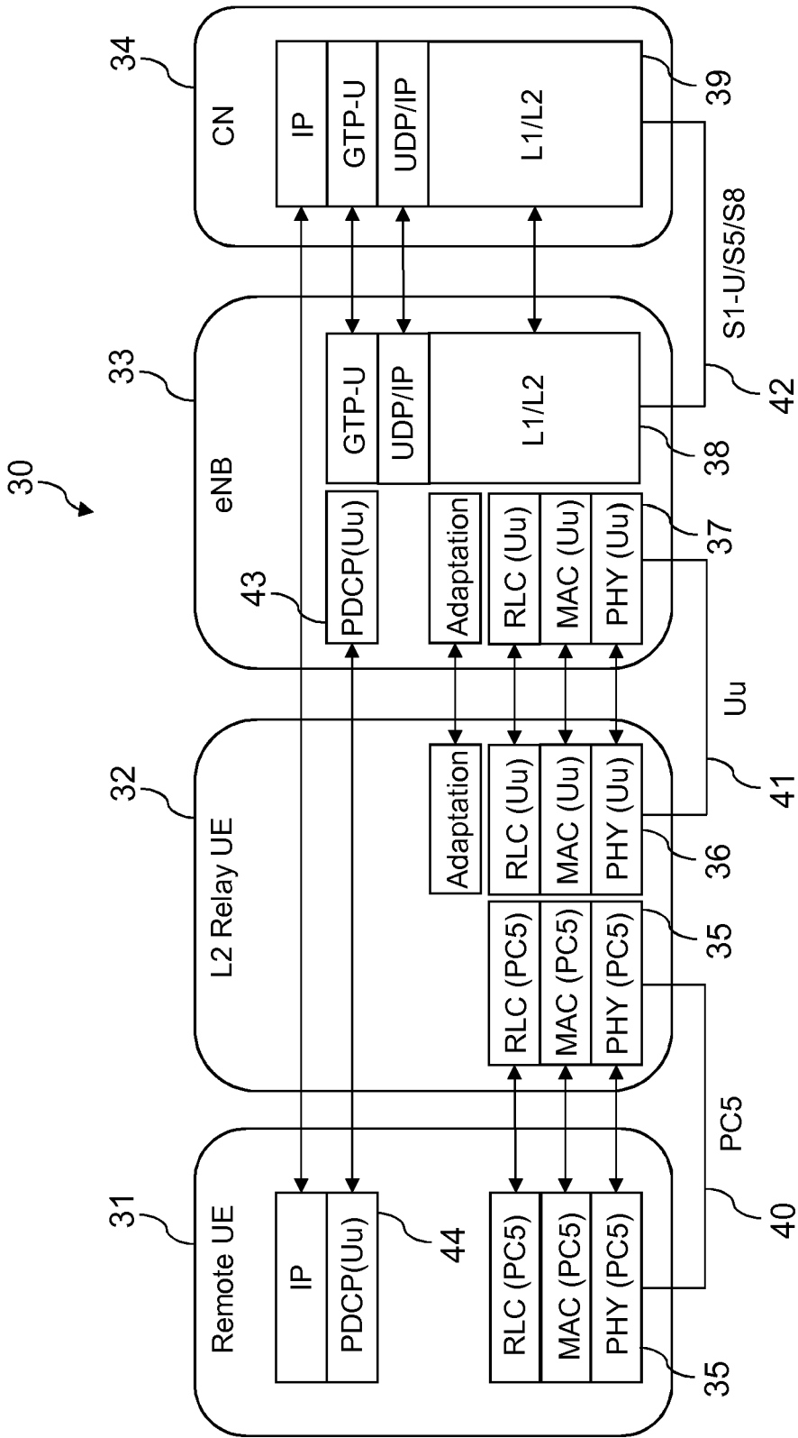
Fig. 2 (prior art)
