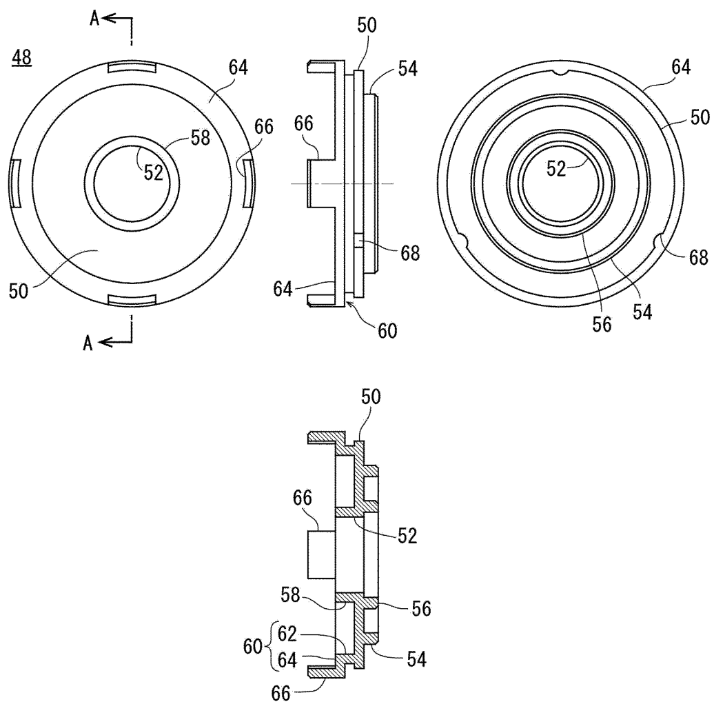
A-A CROSS SECTION
