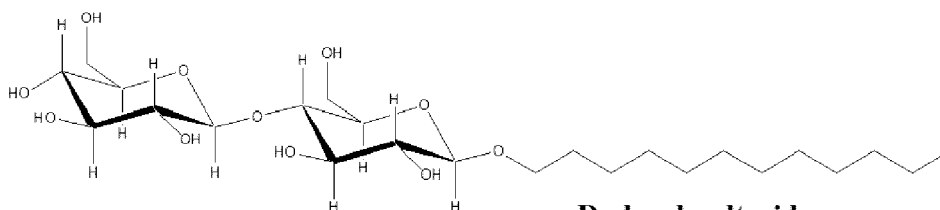
Dodecylmaltoside
