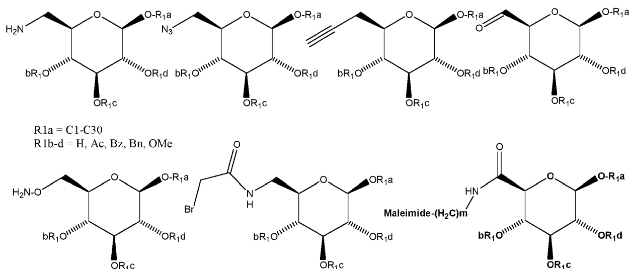
Scheme 6. Additional reagent examples.
