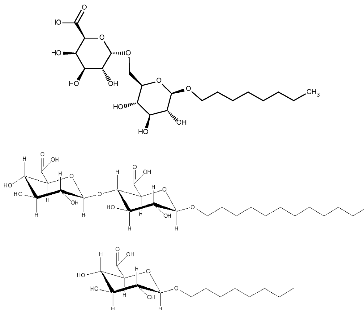
Scheme 2. Examples of alkyl melibiouronic, diglucuronic and glucuronic acid class reagents.
