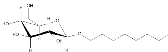
Octylglucoside
