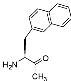
2-(2-naphthyl)-L-alanine (Nal(2))
