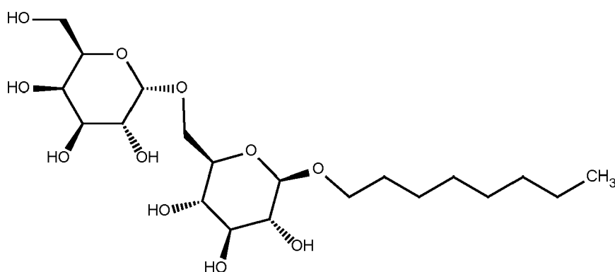
1-Octyl beta-D-melibioside
