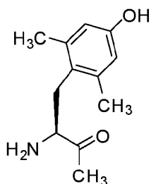
2,6-dimethyl-L-tyrosine (Dmt)
