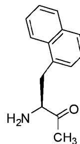
2-(1-naphthyl)-L-alanine (Nal(1))
