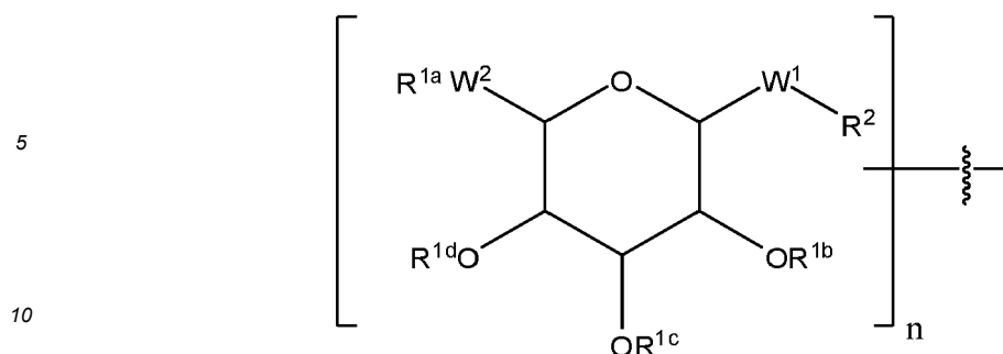
Formula 2-I
