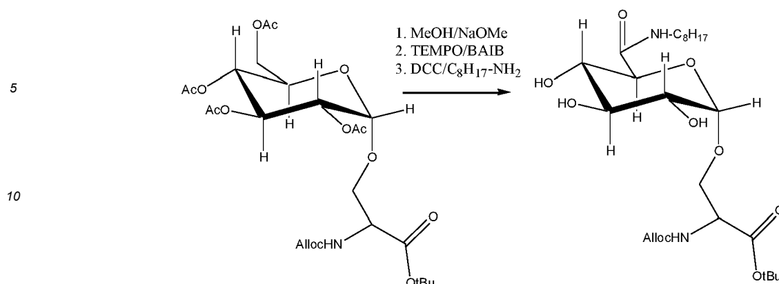
Scheme 7. Alternative example of nonionic surfactant reagent.
