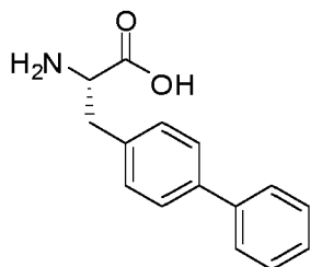
2-L-biphenyl-alanine (Bip)
