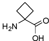
2-aminocyclobutane- 1-carboxylic acid (Ac4c)
