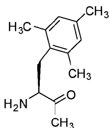
2,4,6-trimethyl-L-phenylalanine (Tmp)
