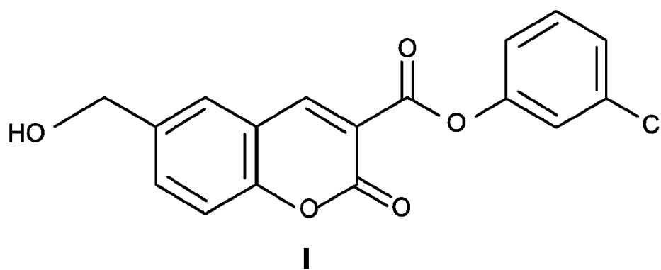
3-(3-chlorophenyl)carboxy-7-hydroxymethyl coumarin
