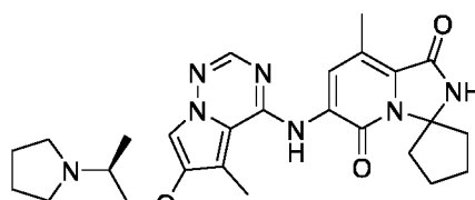
Compound 13
