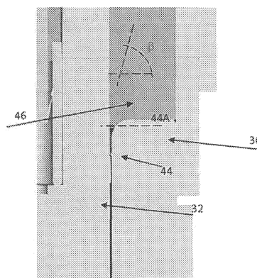
Fig 4 - Detail A of Fig. 3 of the section of the semi- conductive ring (46) with the angle ( \beta ) of contact with the ceramic insulator (32). The metallization height (44A) is recessed with respect of the plug shell (36).
