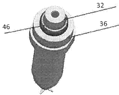
Fig 5 - Firing end: the semi-conductive ring (46) is placed in contact with the ceramic insulator (32) and the metallic shell (36).
