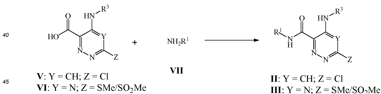
Scheme 2. Coupling of carboxylic acids V/VI with amine VII
