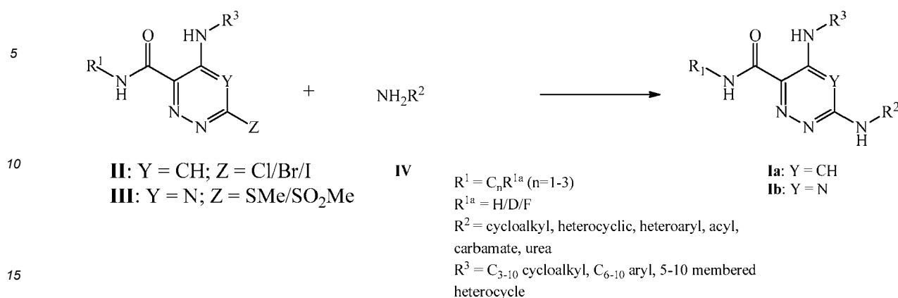
Scheme 1. Coupling of II/III with amine IV
