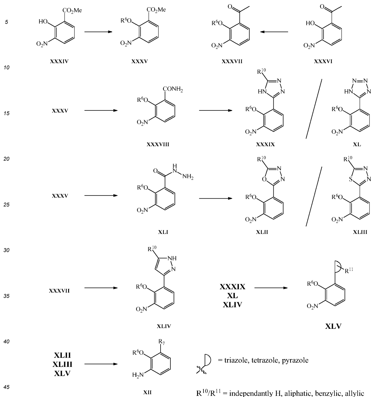
Scheme 12. Alternate synthesis of anilines XII
