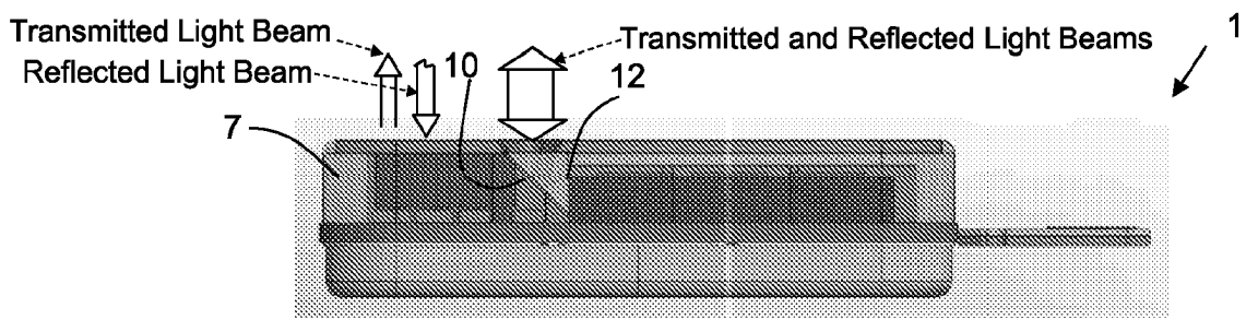
FIG. 1C Cross section view with lid shown
