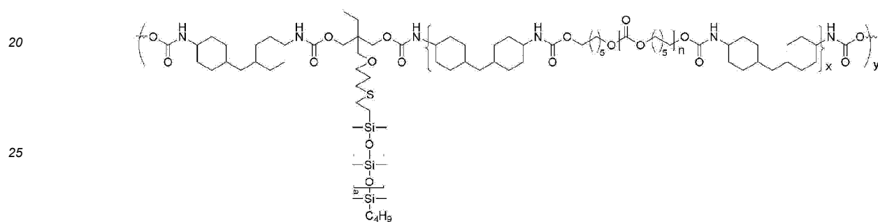
[Chemical formula 8]
