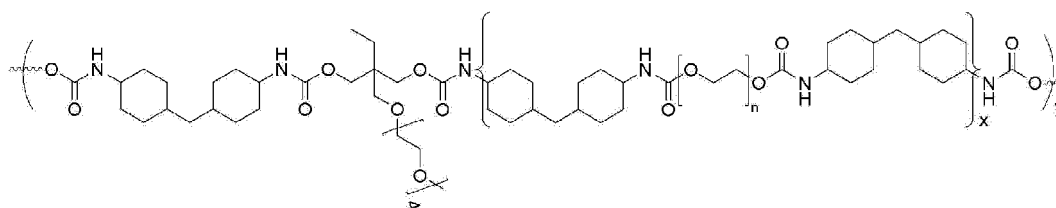
[Chemical formula 2]
