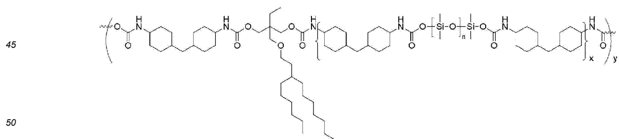
[Chemical formula 9]
