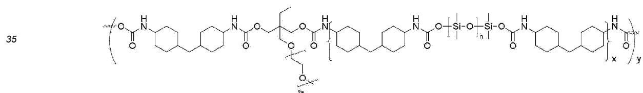
[Chemical formula 9]
