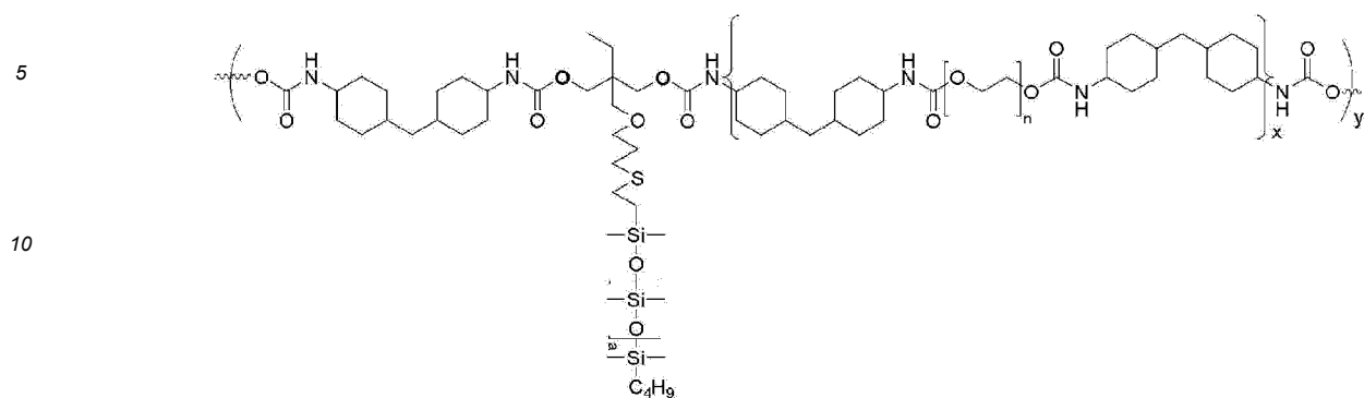
[Chemical formula 7]
