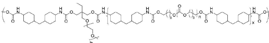
[Chemical formula 5]
