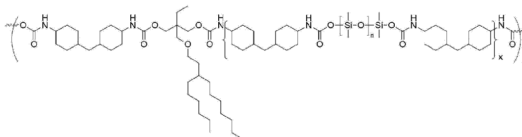
[Chemical formula 9]
