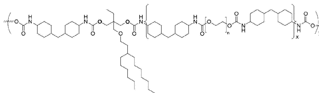
[Chemical formula 4]
