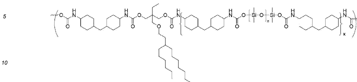
[Chemical formula 9]
