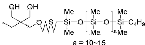
[Chemical formula 13]
