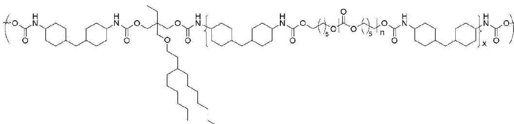
[Chemical formula 5]
