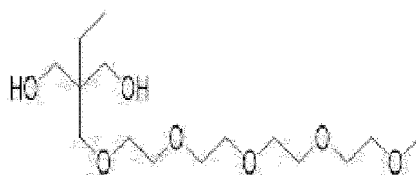
[Chemical formula 12]
