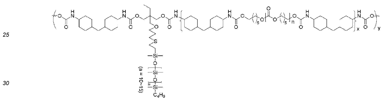
[Chemical formula 7]
