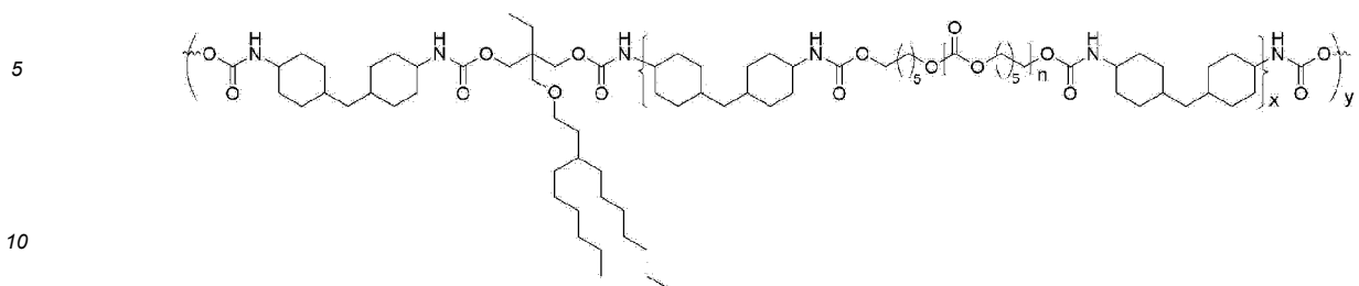
[Chemical formula 6]
