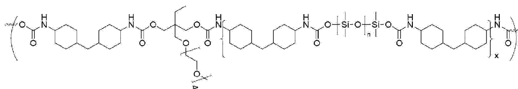
[Chemical formula 9]
