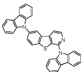
Compound 4
