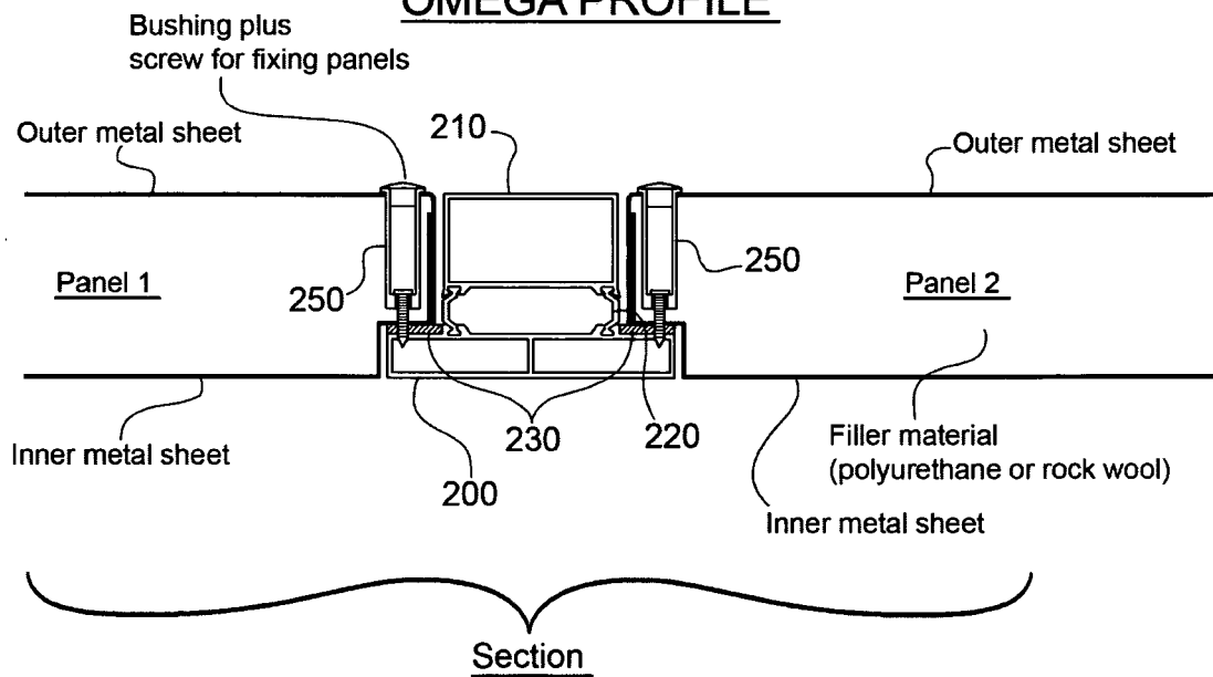
FIG.5 (PRIOR ART) OMEGA PROFILE
