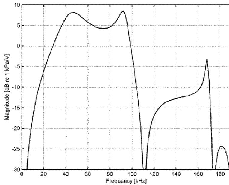
Transmission Sensitivity
