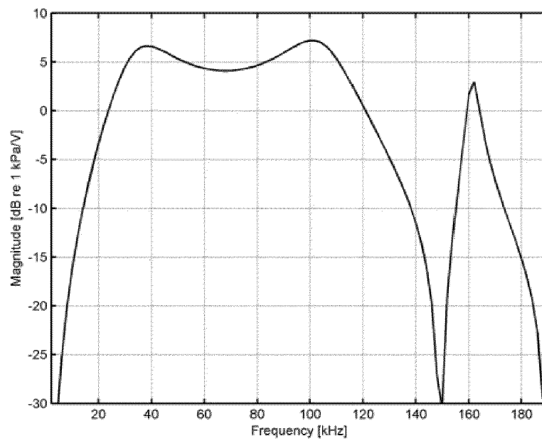
Transmission Sensitivity
