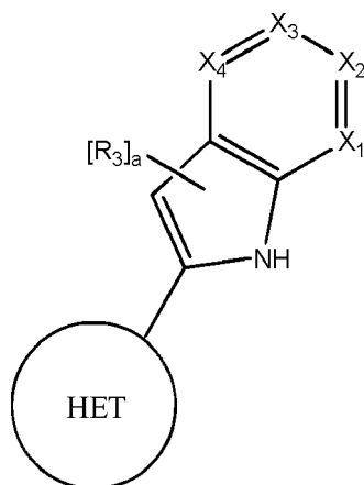
Formula I
