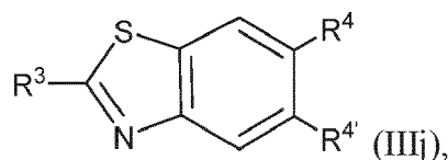
(IIIi),
