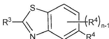
(IIIc),
