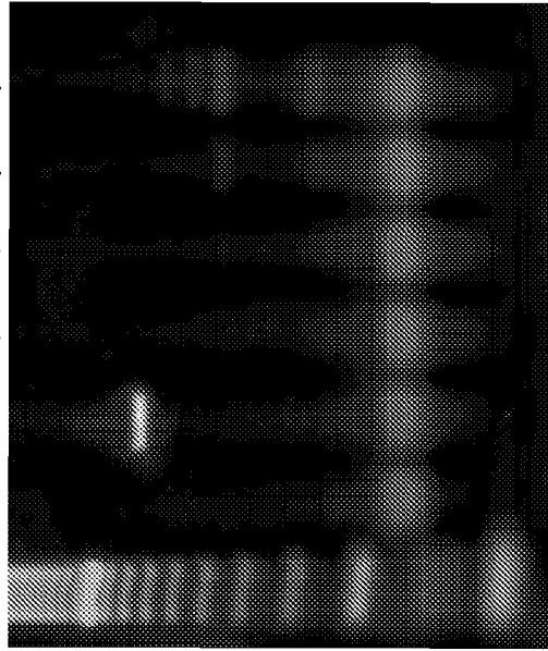
Fig. 34A Enzyme mix only +full record (10fM) +1p M SPEED Probe +10 pM SPEED Probe +100 pM SPEED Probe +1 nM SPEED Probe
