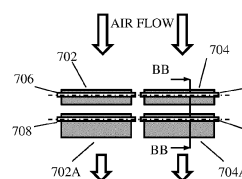
Fig. 7B CROSS SECTION AA
