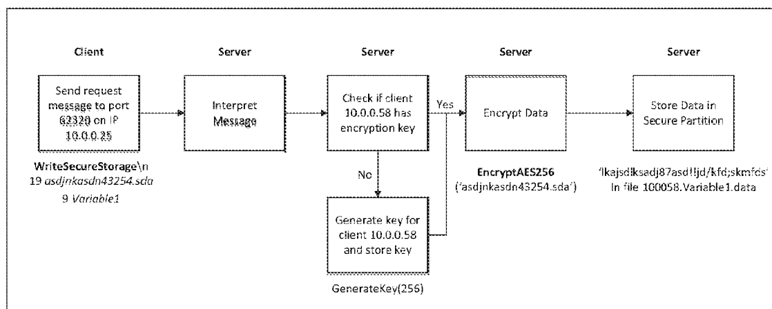
Figure 11. Secure storage service request example
