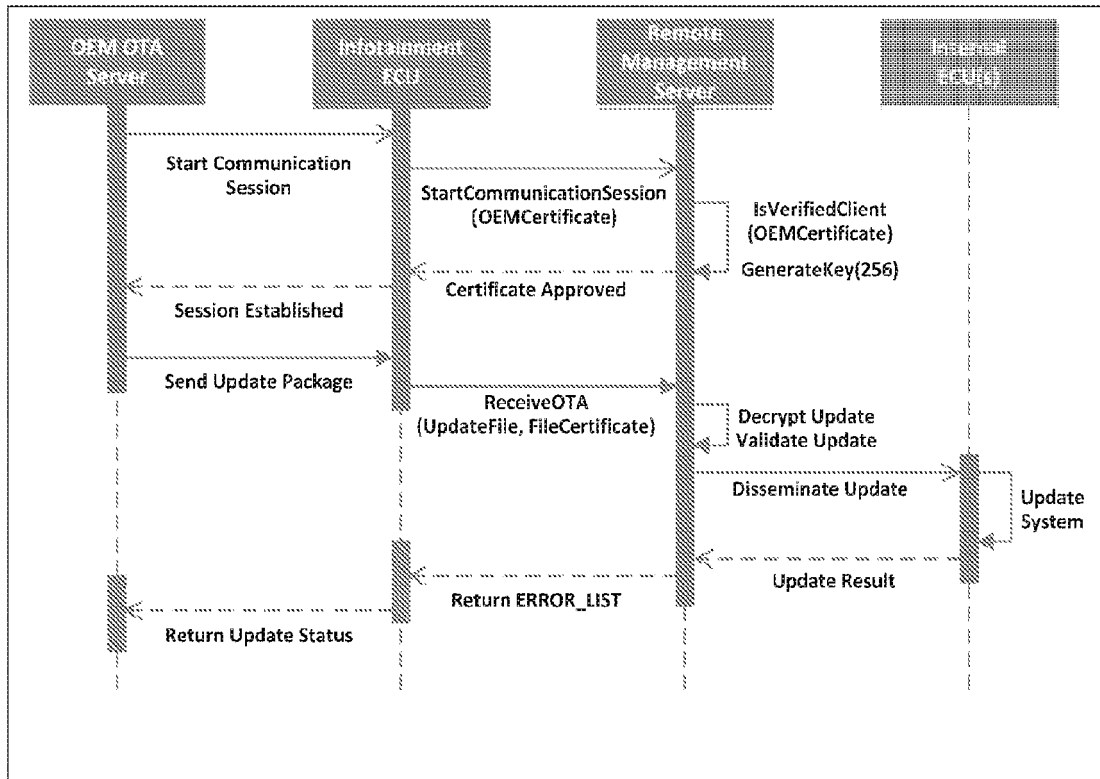
Figure 7. OTA process example using remote management ECU services
