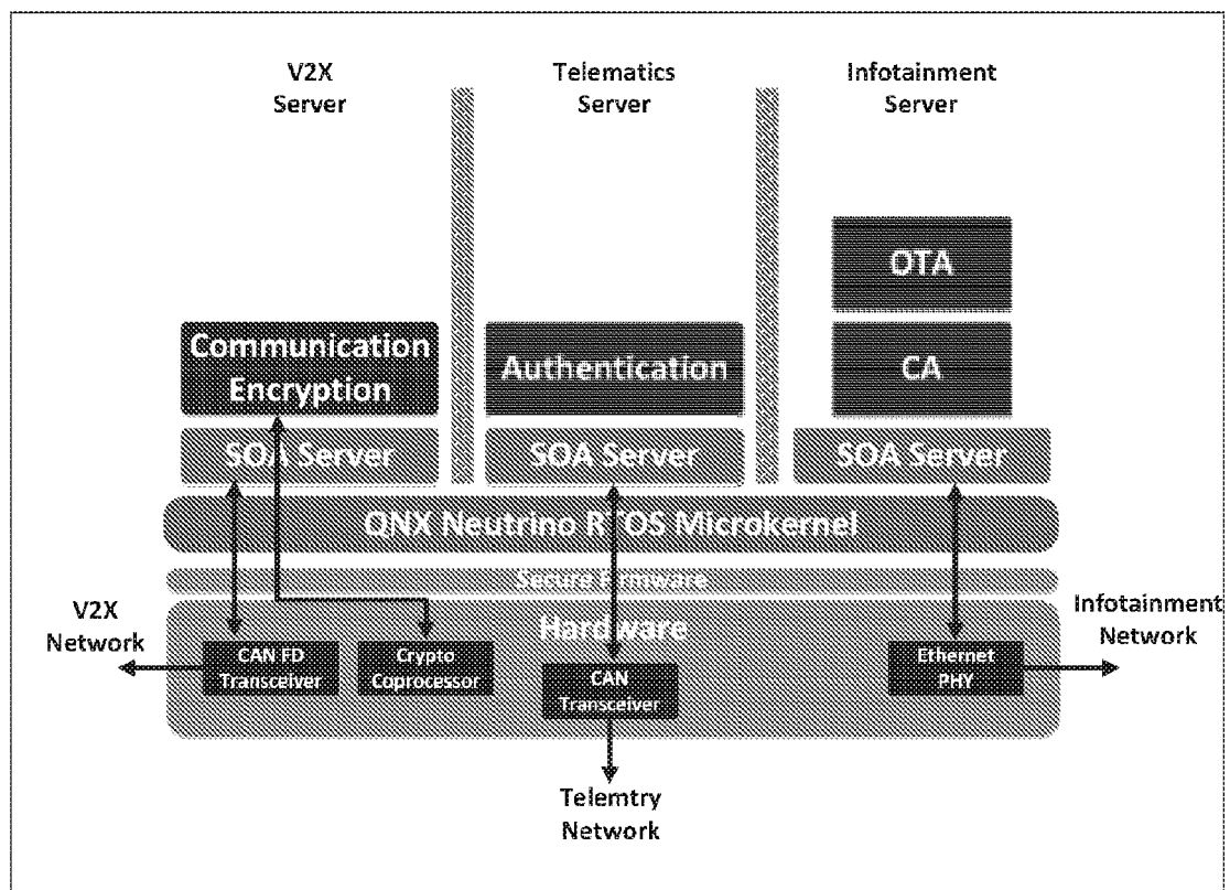
Figure 6. Remote management server software architecture
