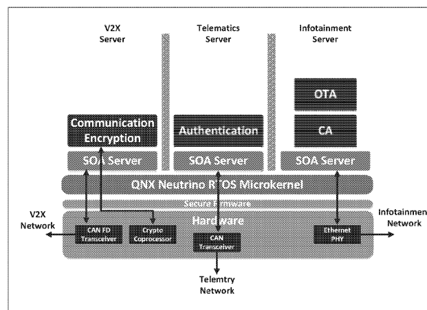
Figure 6. Remote management server software architecture
