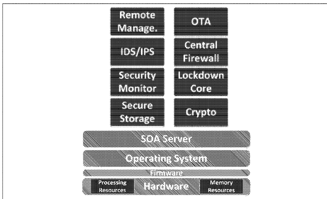
Figure 1. Centralized inventive SOA ECU architecture example
