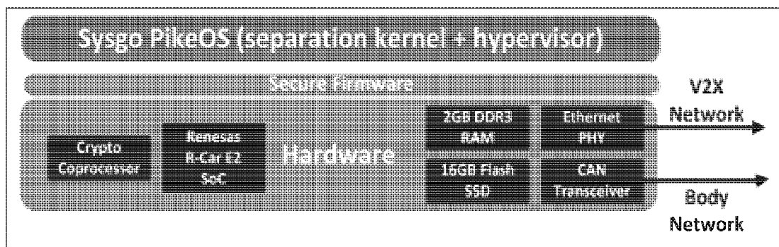
Figure 9. Example security server ECU architecture
