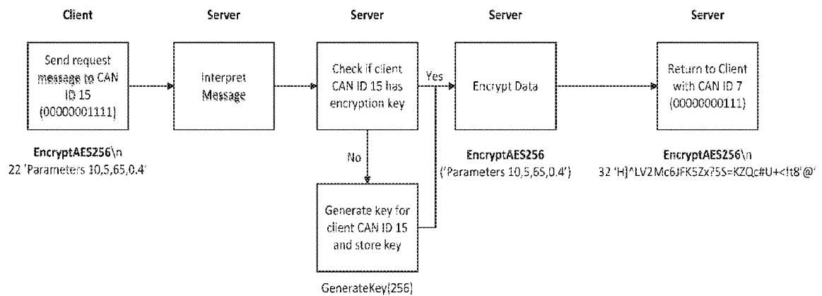
Figure 8. Communication encryption service request example
