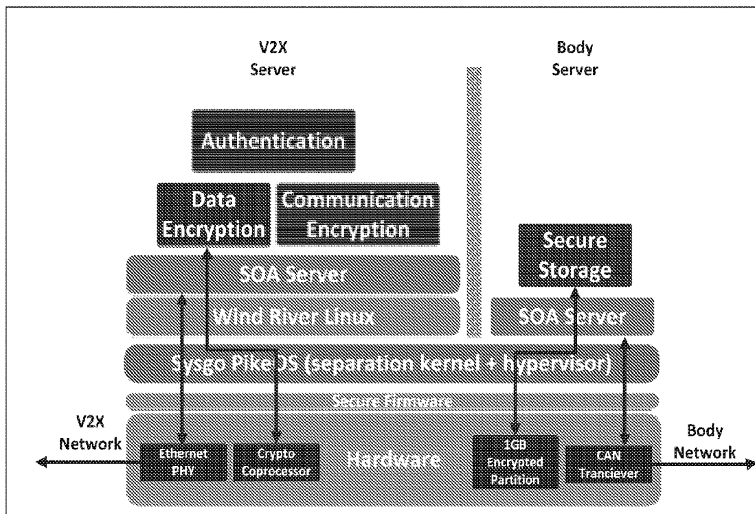
Figure 10. The inventive SOA security server architecture example
