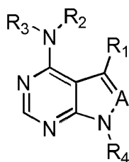
Formula (A);
