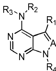
Formula (A);
