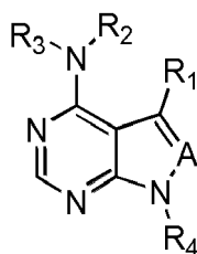
Formula (A)
