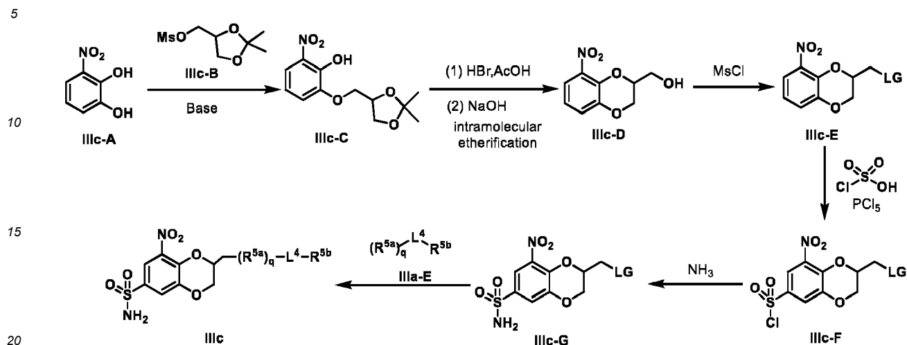
Scheme 4
