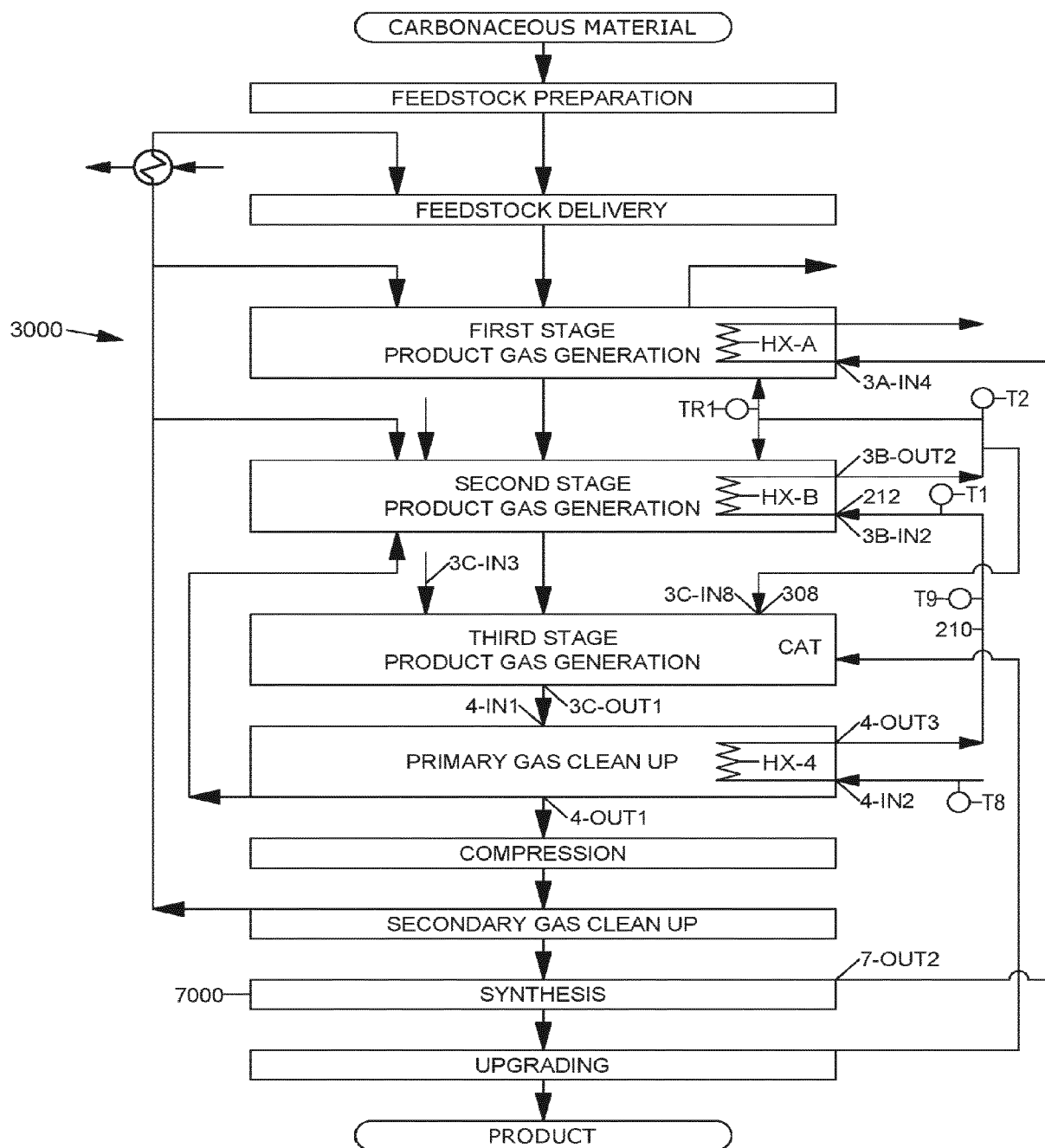
FIGURE 26 REFINERY SUPERSTRUCTURE (RSS)
