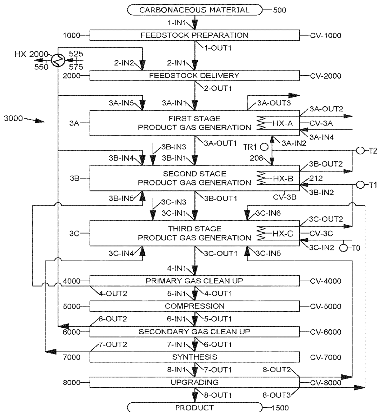
FIGURE 25 REFINERY SUPERSTRUCTURE (RSS)
