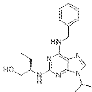
Seliciclib Chemical Structure
