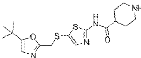
SNS032 Chemical Structure
