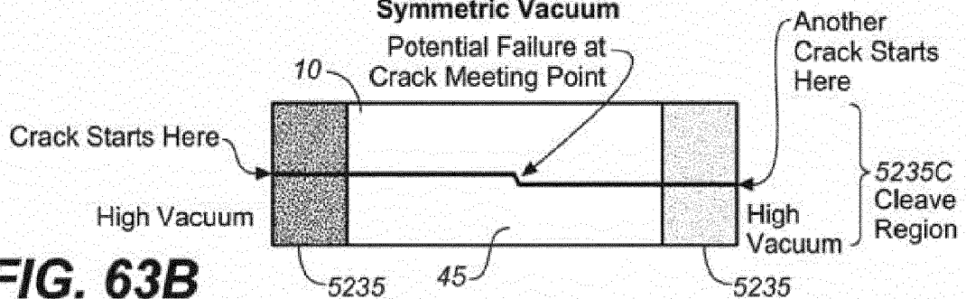
Symmetric Vacuum
