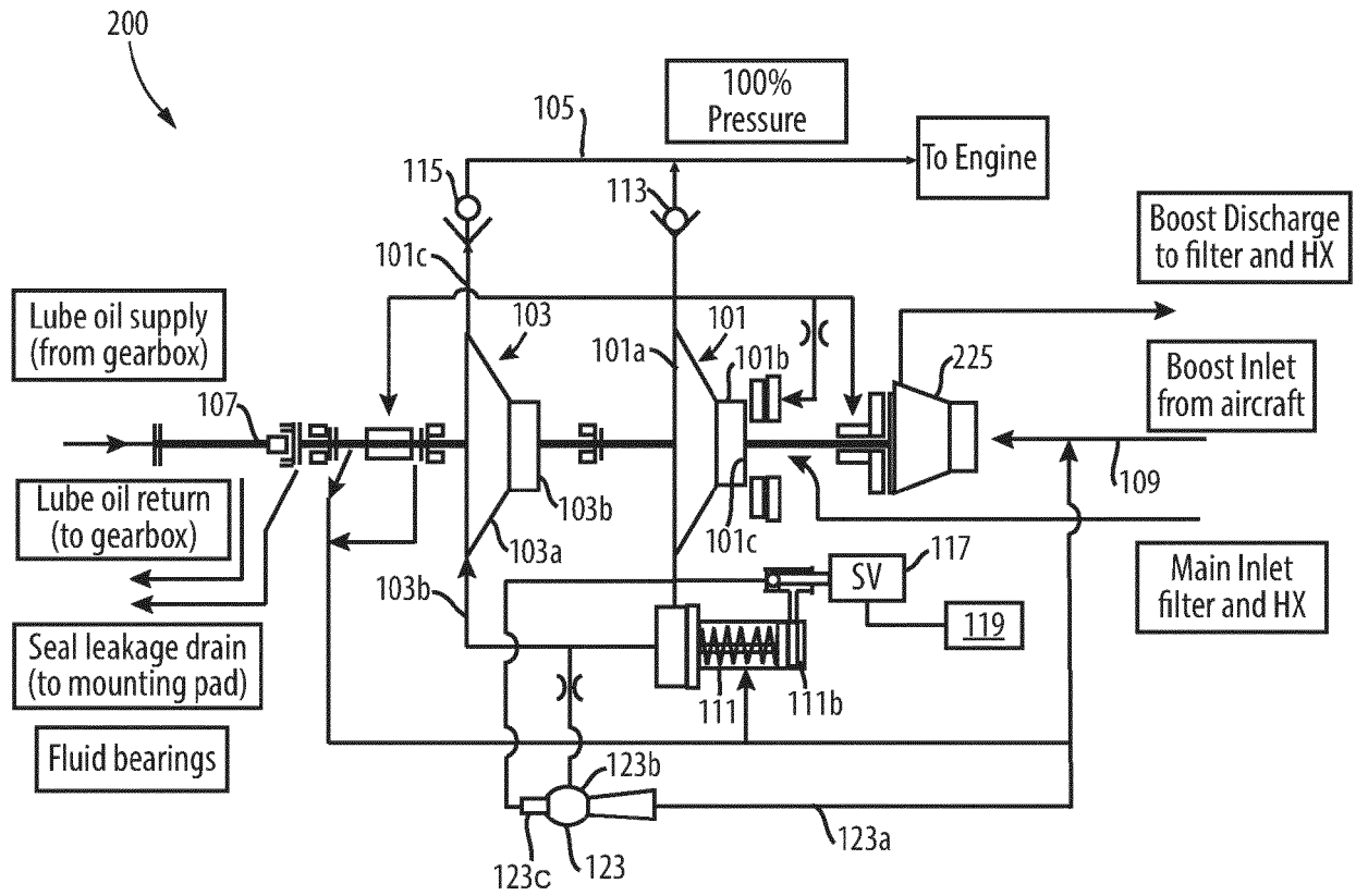
2 Stage Operating Mode
