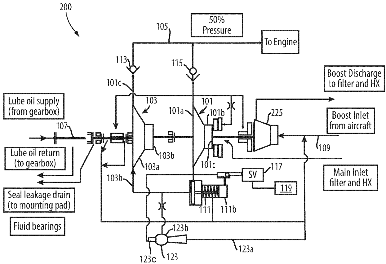
Dry 2nd Stage at Idle and Cruise
