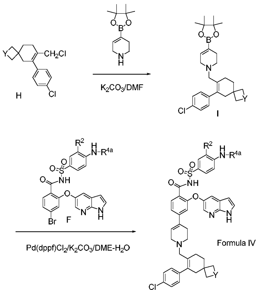
General Scheme 4
