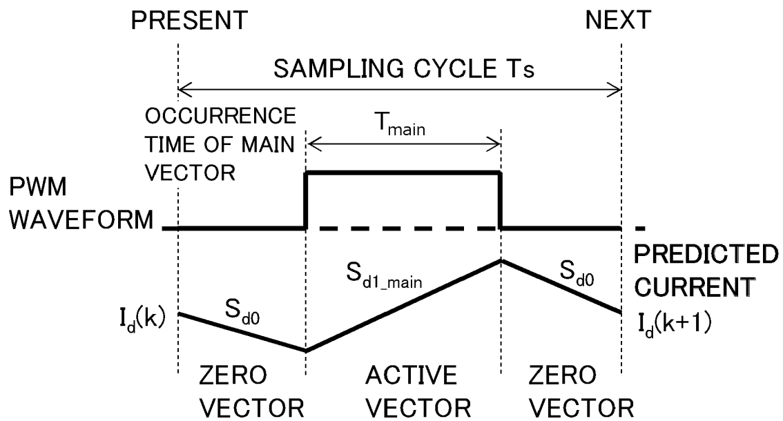
EXAMPLE OF d-AXIS CURRENT
