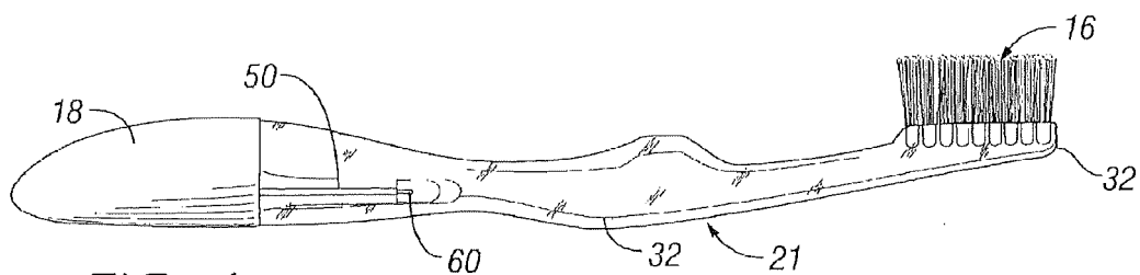
FIG. 4 (PRIOR ART)
