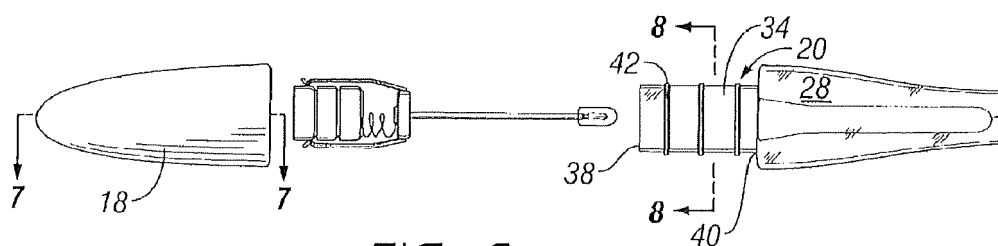
FIG. 6 (PRIOR ART)
