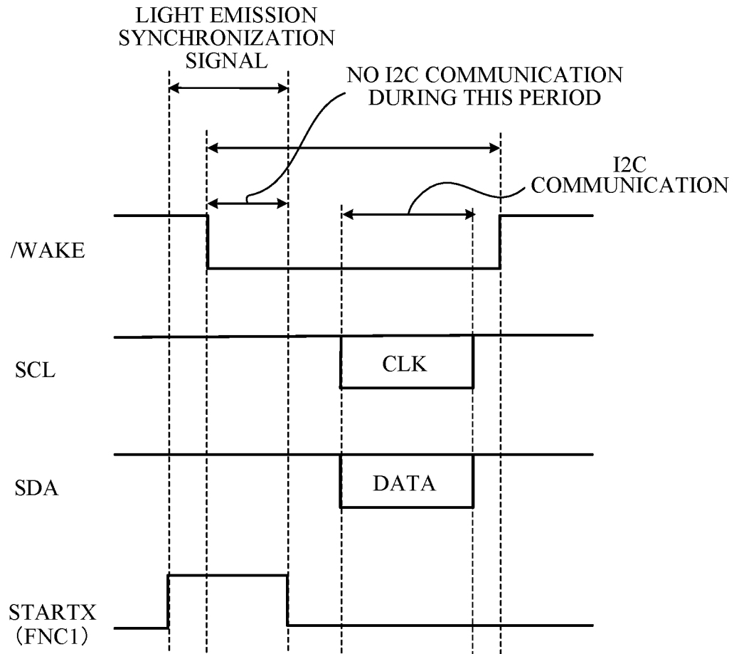
COMMUNICATION REQUEST ( \overline{\text{WAKE}} ) AND I2C AND STROBO LIGHT EMISSION TIMING
