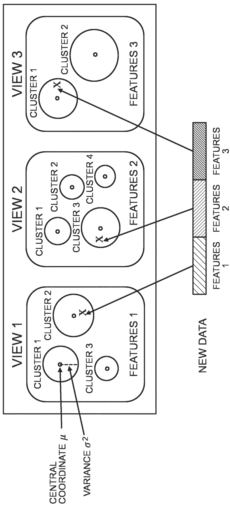
Fig. 48 CLUSTERING CLASSIFIER
