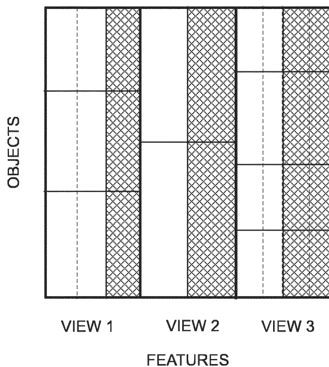
Fig. 23 MULTIPLE CO-CLUSTERING
