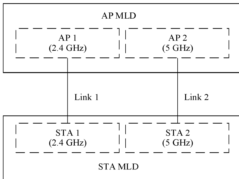
Communication system 200
