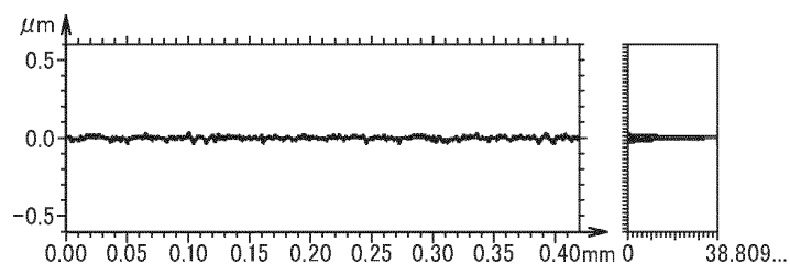
FIG. 6A BALL SURFACE
