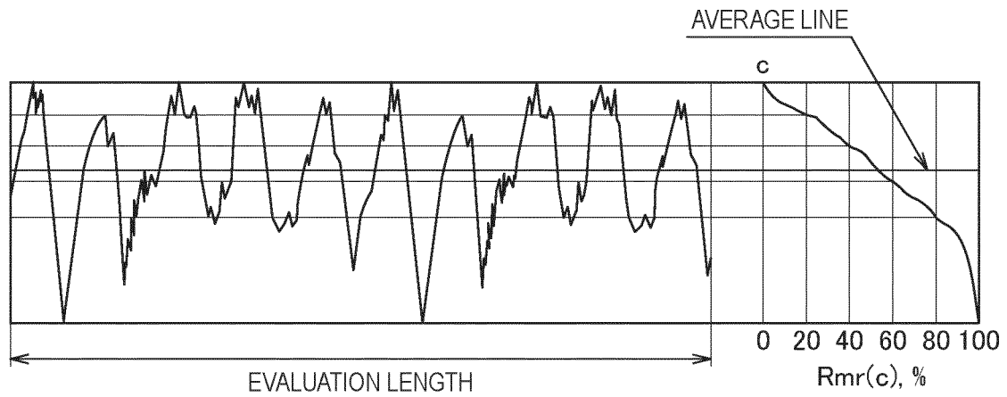
ROUGHNESS CURVE AND MATERIAL RATIO CURVE THEREOF
