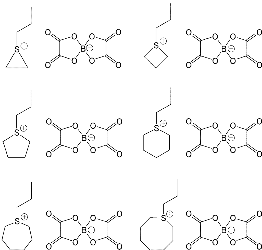
[Chem. 9]
