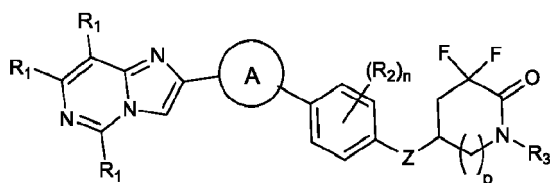
Formula (IIId);
