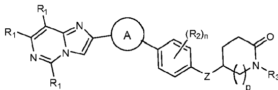
Formula (Id);
