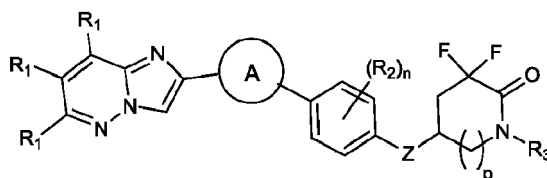
Formula (IIe);
