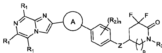
Formula (IIc);
