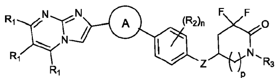
Formula (IIb);
