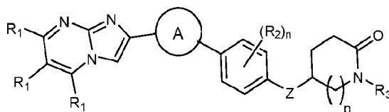
Formula (Ib);
