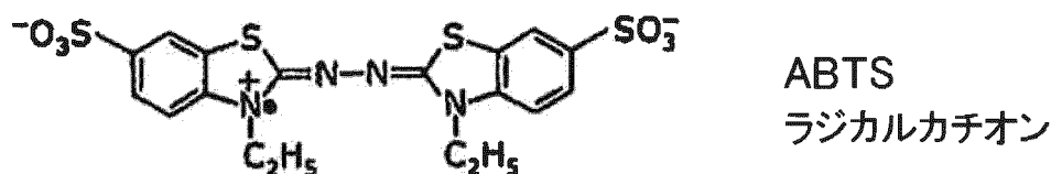
ABTS Radical Cation
