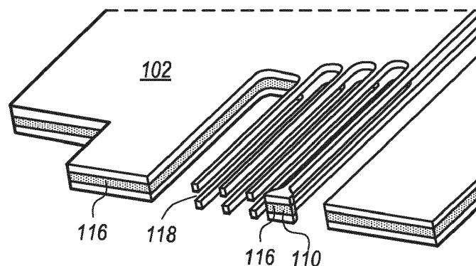
Section B-B FIG. 1C
