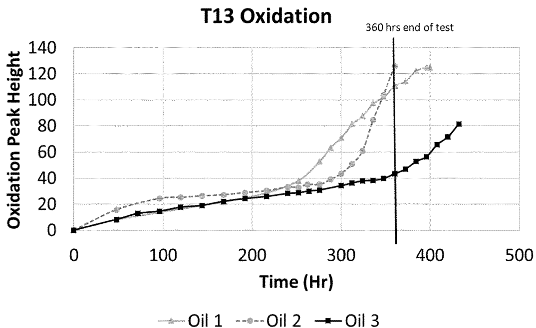
Figure 2 – Oxidation peak heights measured during Worked Example 2
