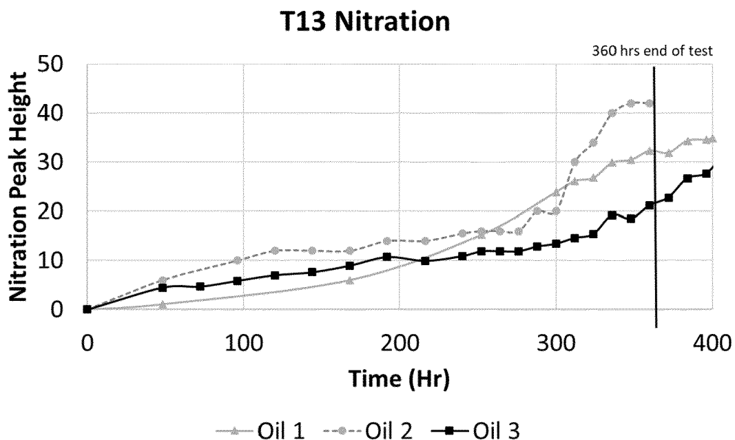
FIGURE 1 – Nitration peak heights measured during Worked Example 2
