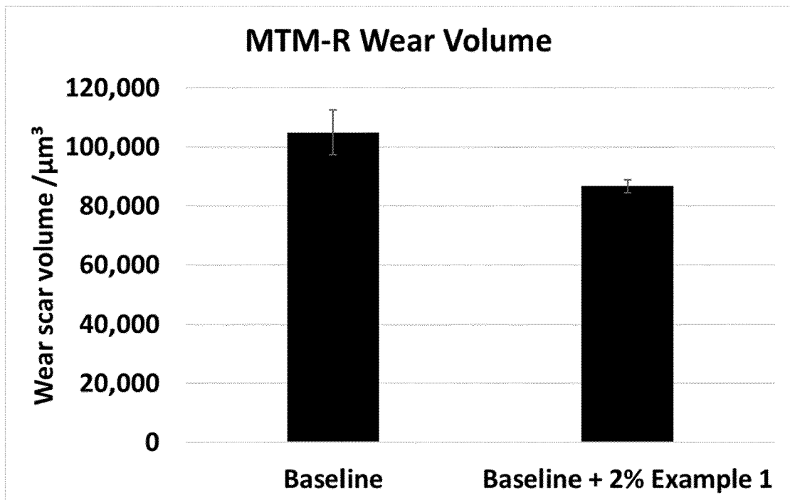
Figure 6 – Wear Scar volume tests by MTM-R
