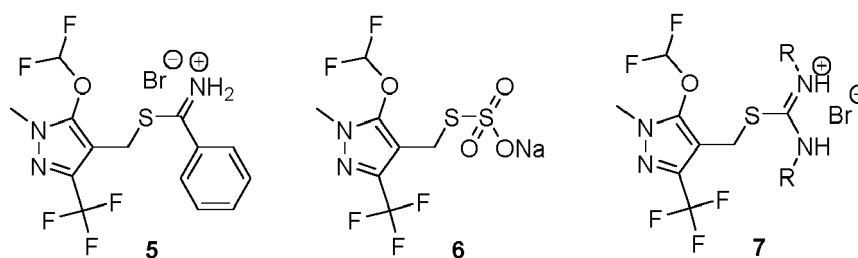
[0033] Figure 3. Products of Step b. (Pyroxasulfone synthesis).
