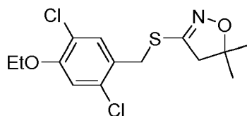
Fenoxasulfone immediate precursor
