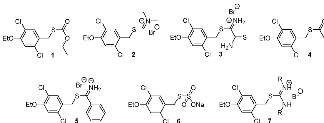
[0036] Figure 4. Products of Step b. (Fenoxasulfone synthesis).
