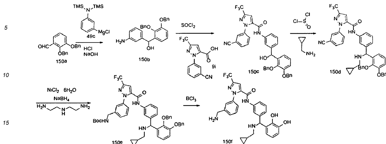
Scheme 150
