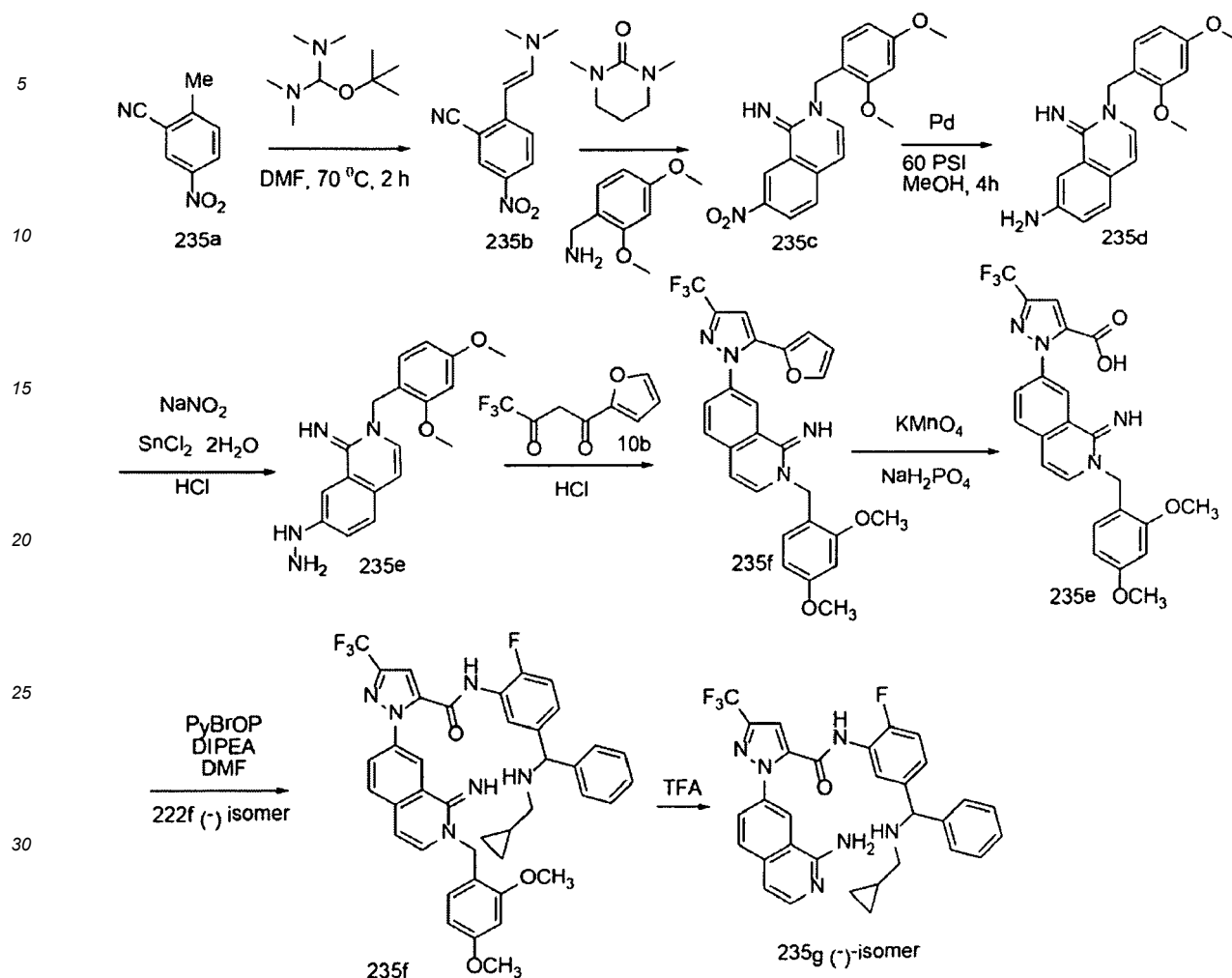
Scheme 235
