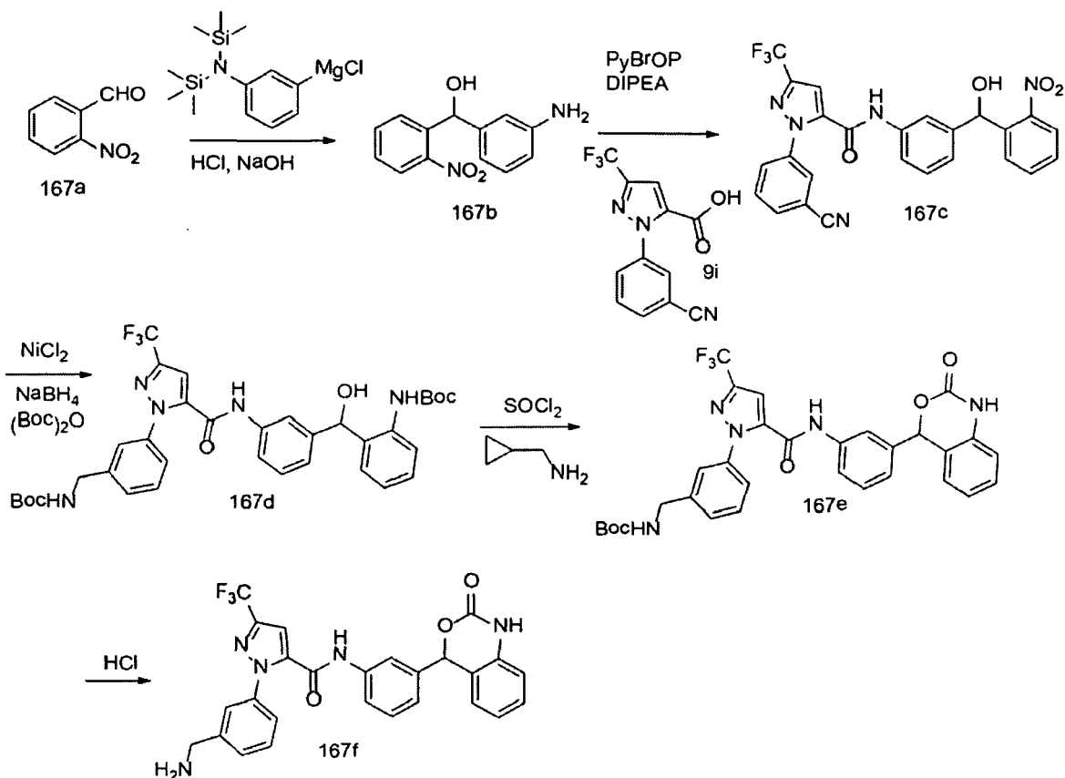
Scheme 167
