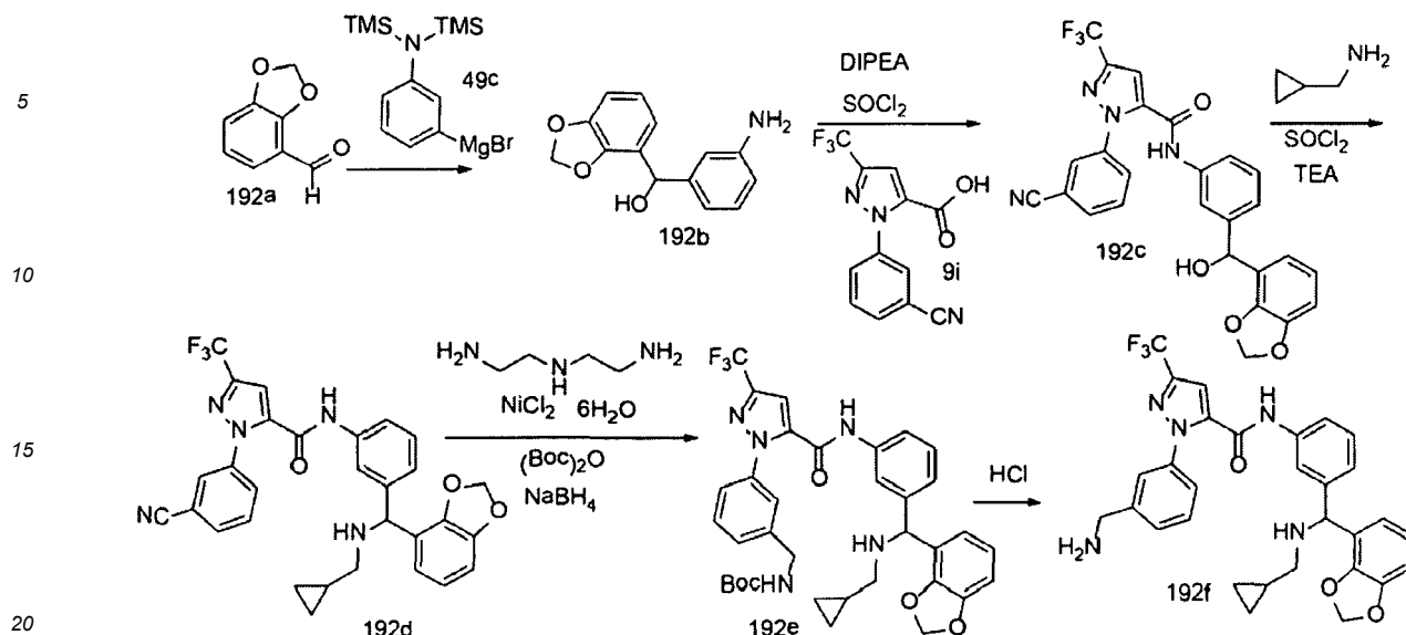
Scheme 192
