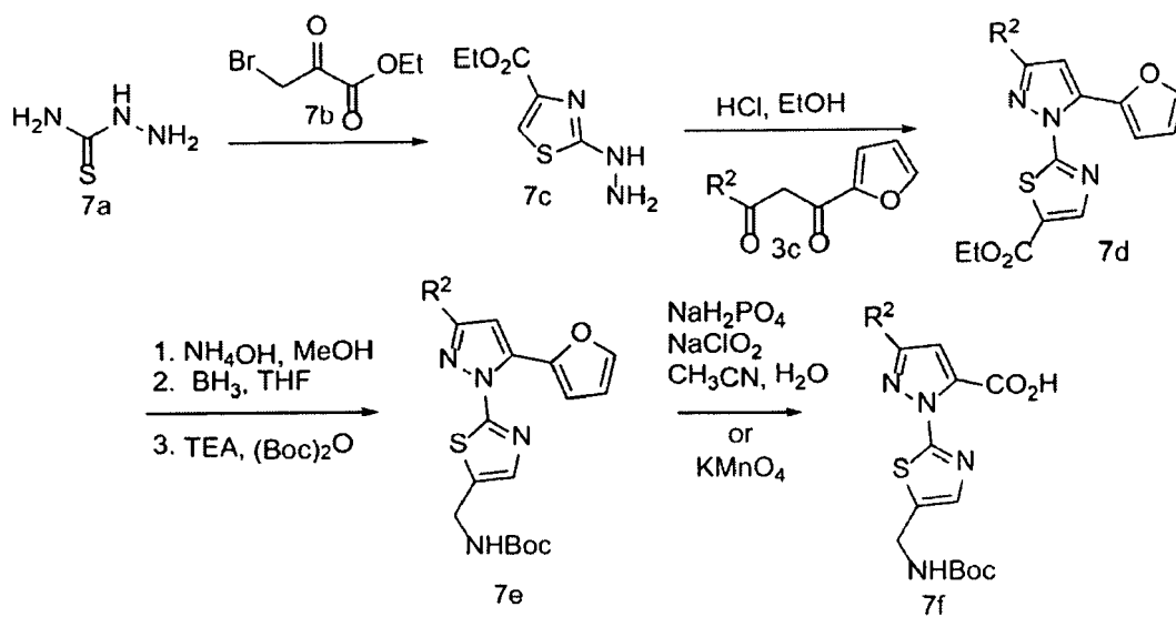
Scheme 7
