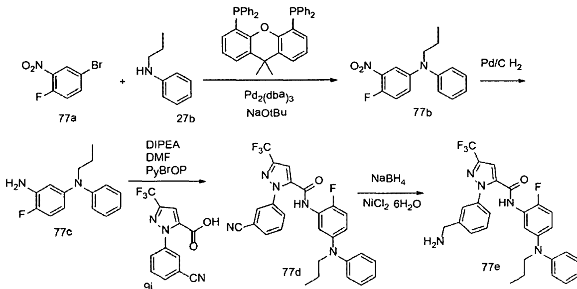
Scheme 77
