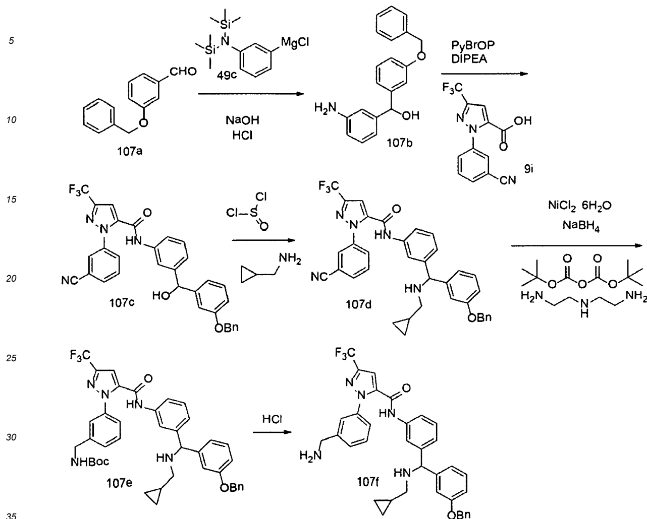
Scheme 107
