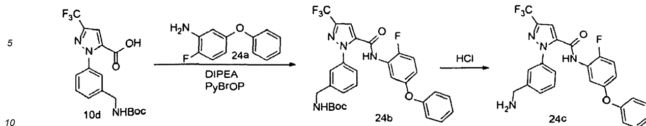
Scheme 24
