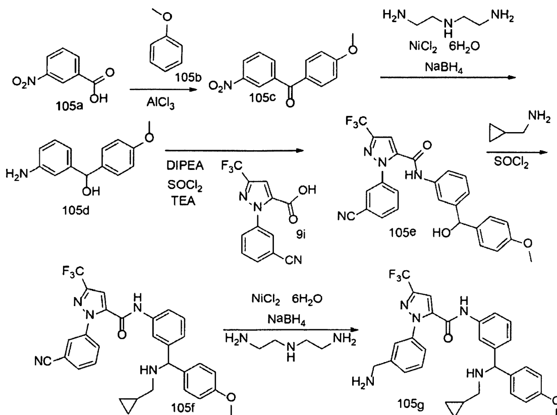
Scheme 105
