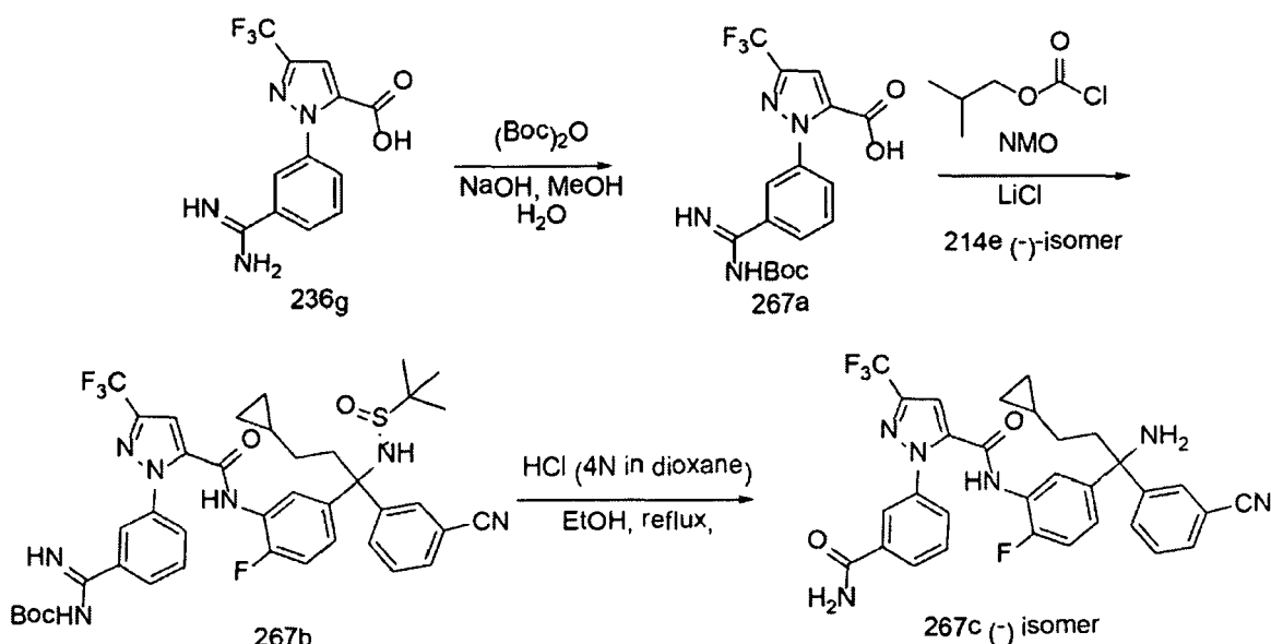
Scheme 267
