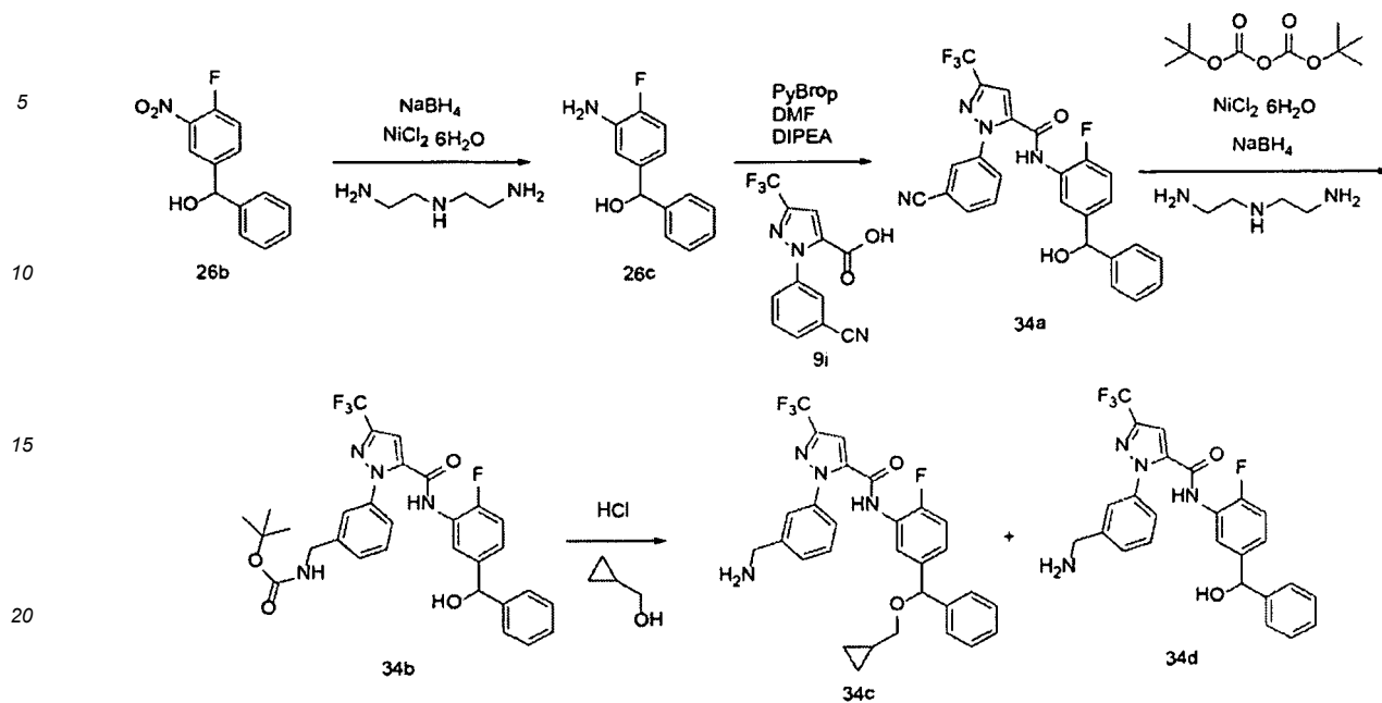
Scheme 34
