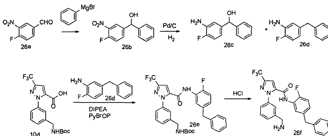
Scheme 26
