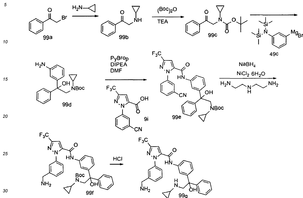
Scheme 99
