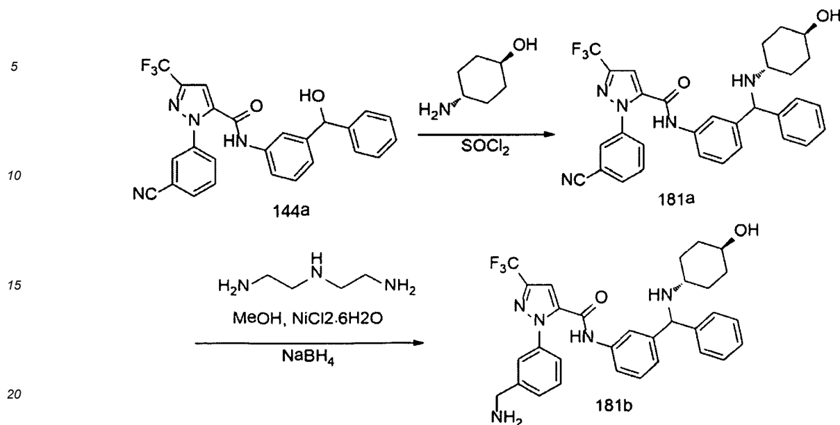
Scheme 18I
