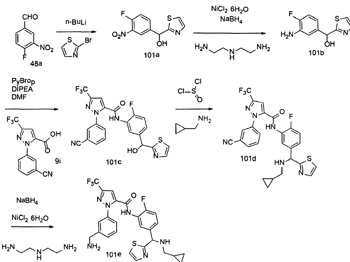
Scheme 101
