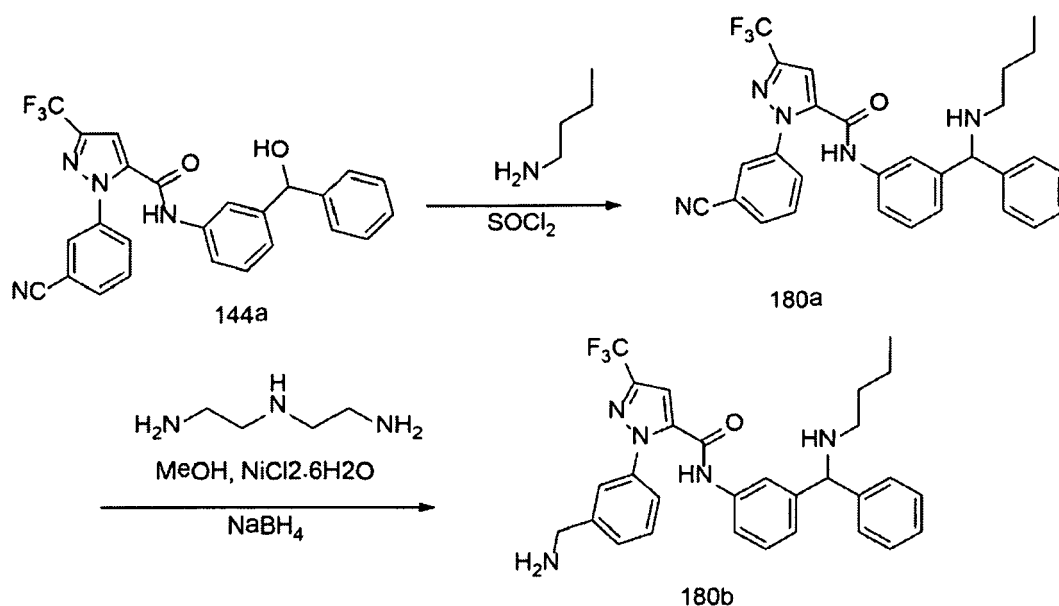
Scheme 180
