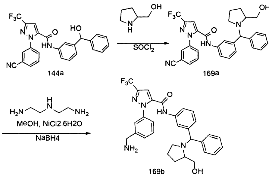
Scheme 169
