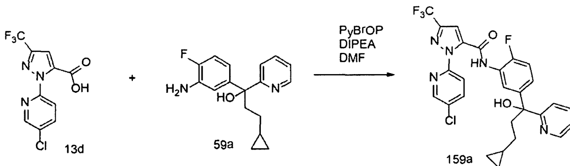
Scheme 159
