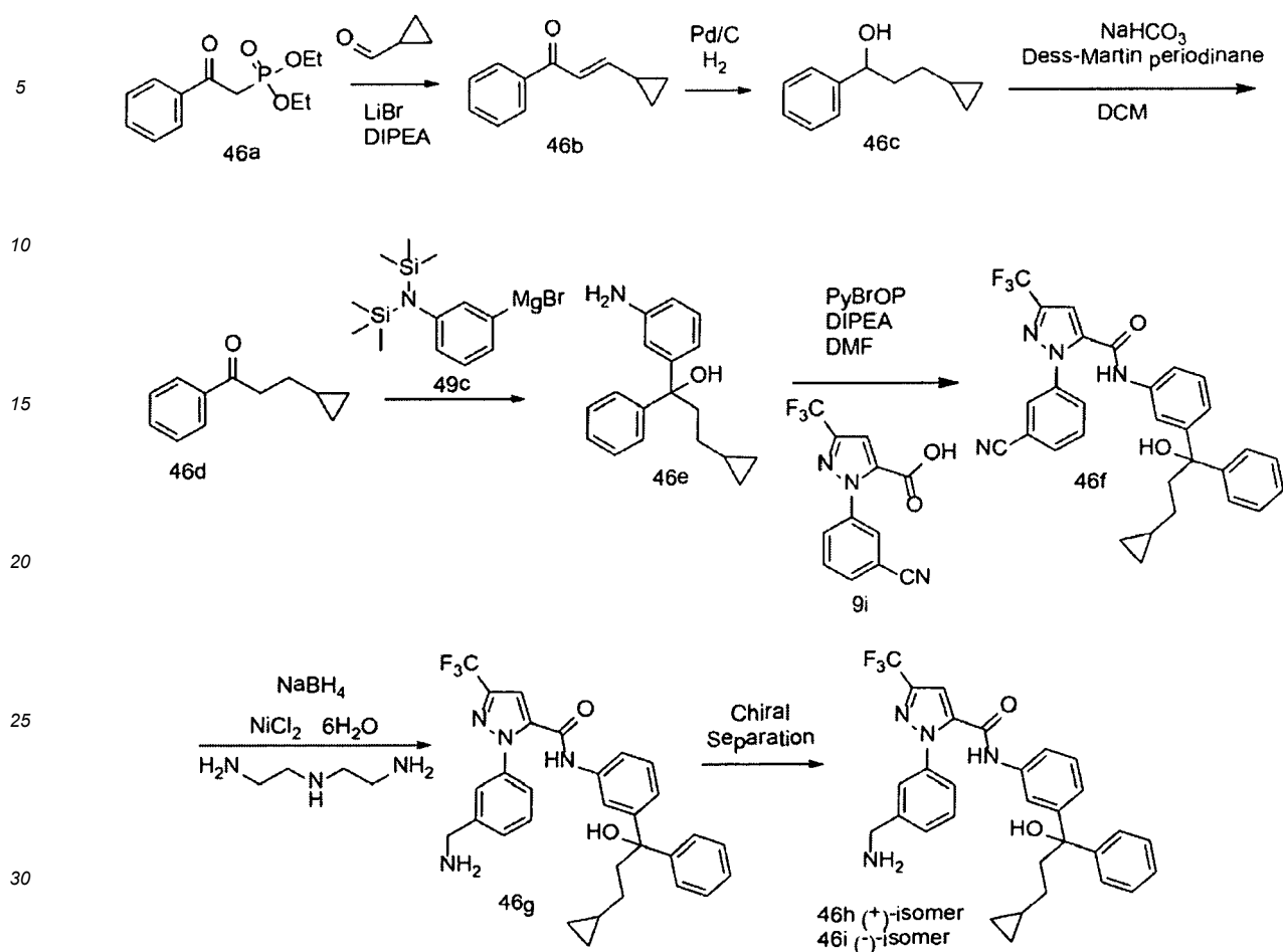
Scheme 46
