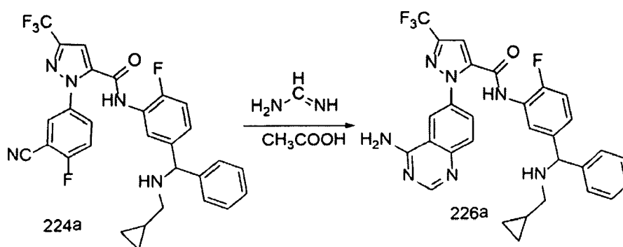
Scheme 226
