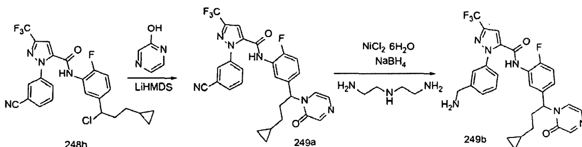
Scheme 249
