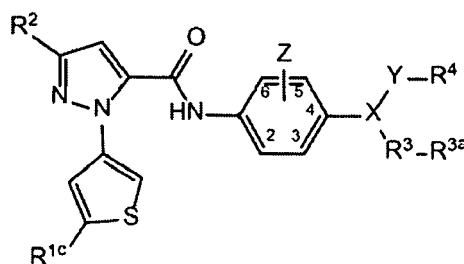
(XXIII)
