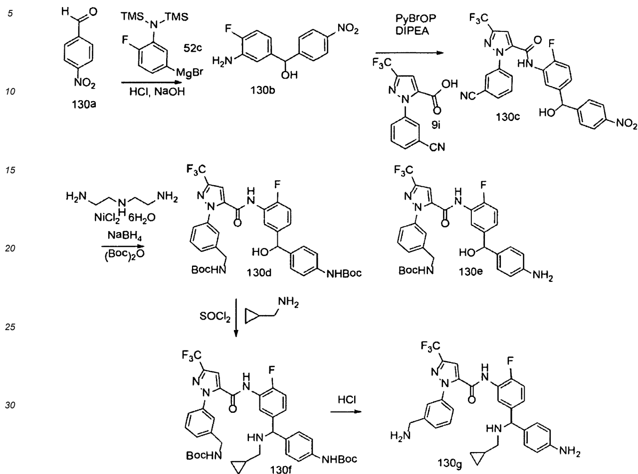
Scheme 130
