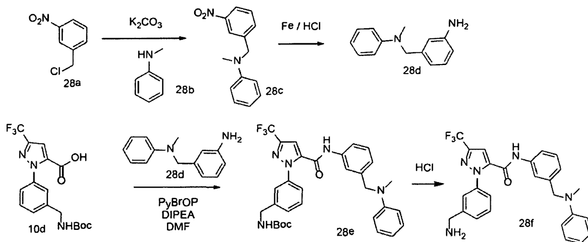
Scheme 28
