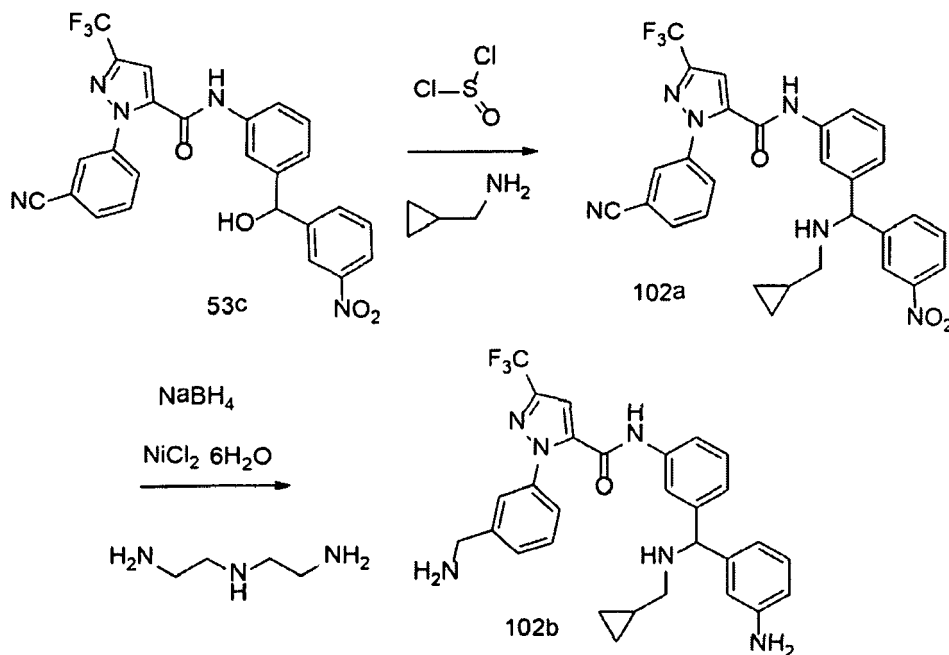
Scheme 102
