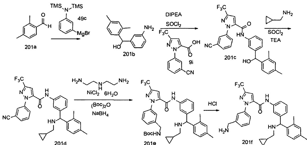
Scheme 201
