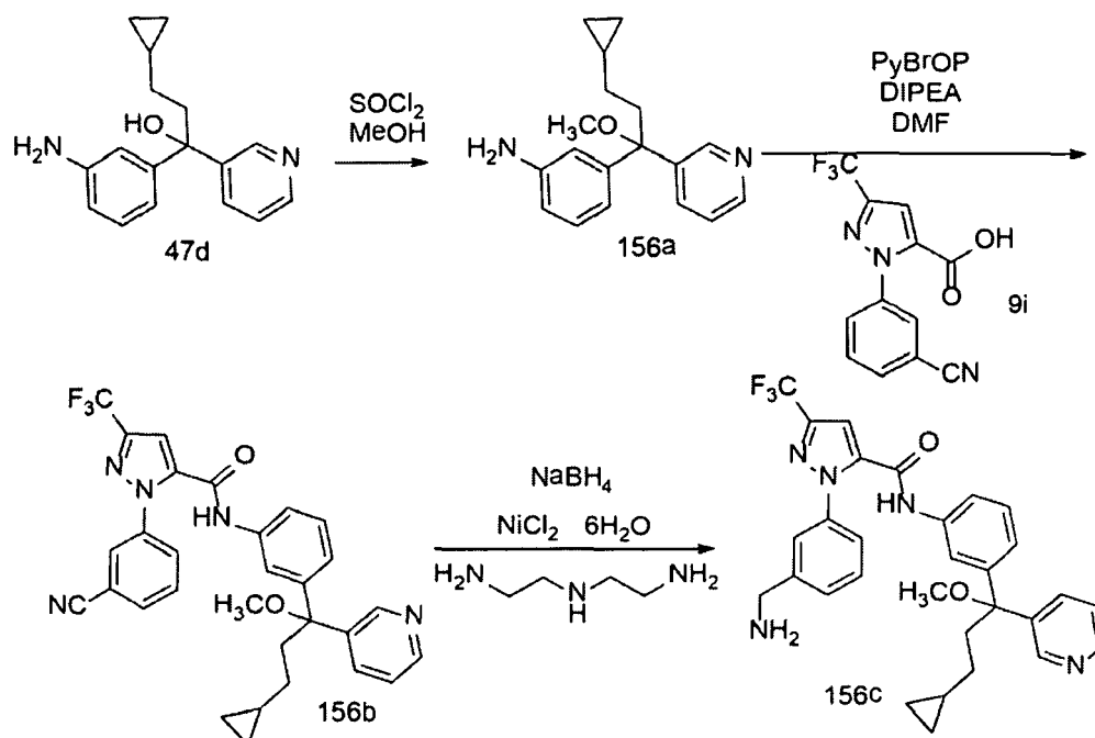
Scheme 156
