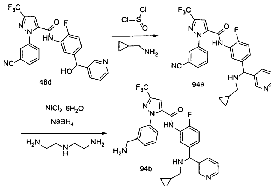
Scheme 94
