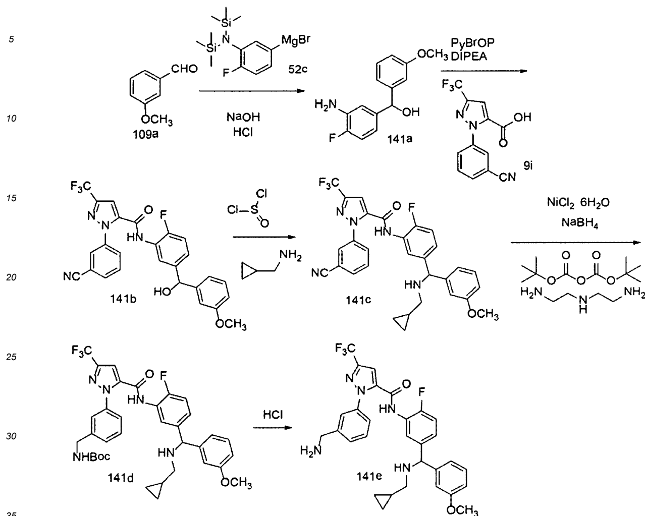
Scheme 141
