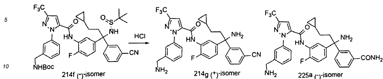
Scheme 225
