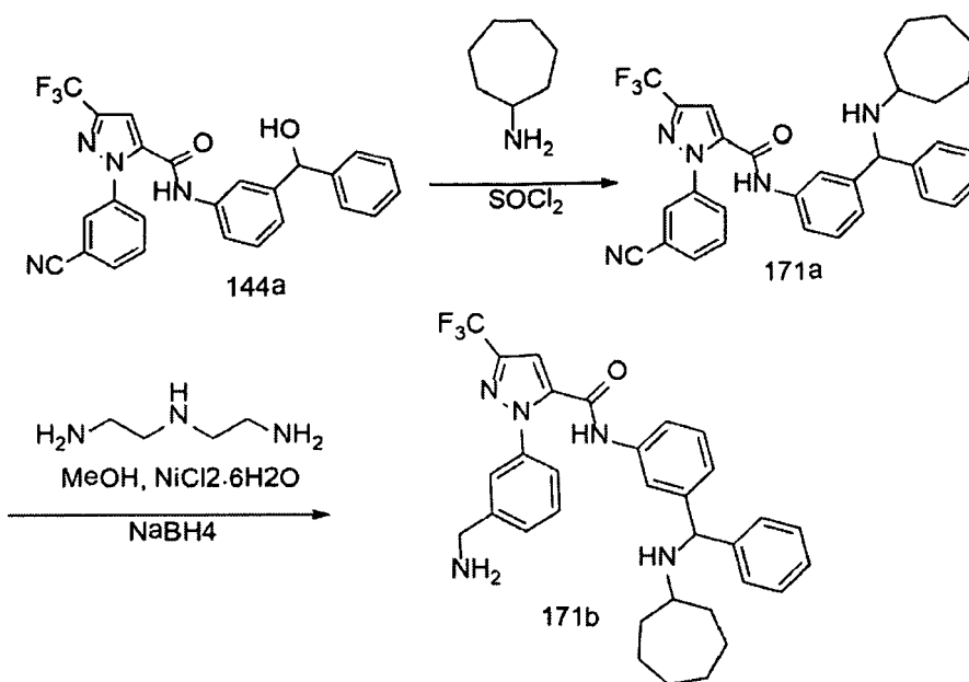
Scheme 171
