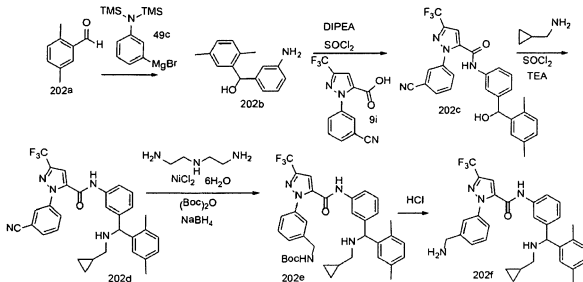
Scheme 202
