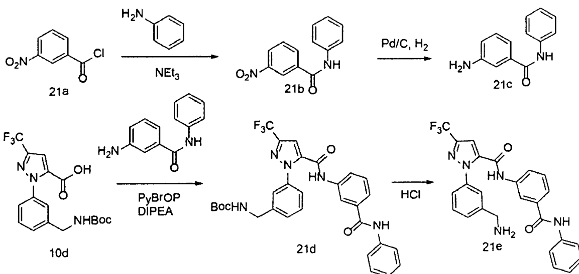
Scheme 21
