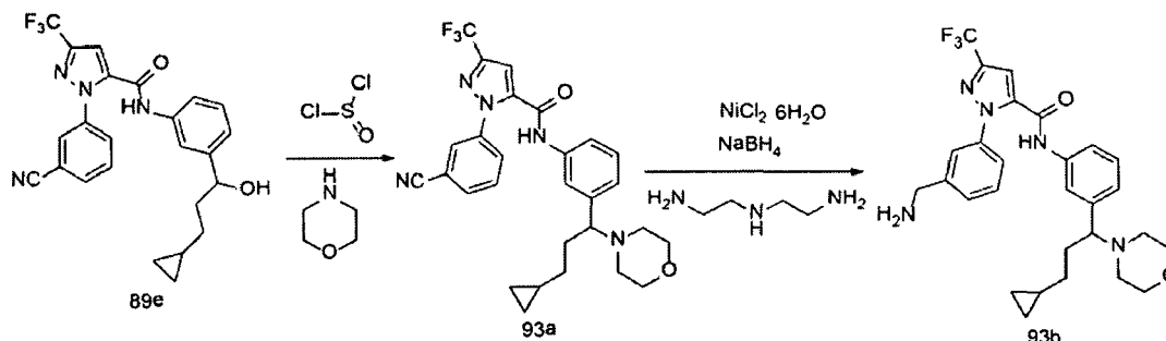
Scheme 93
