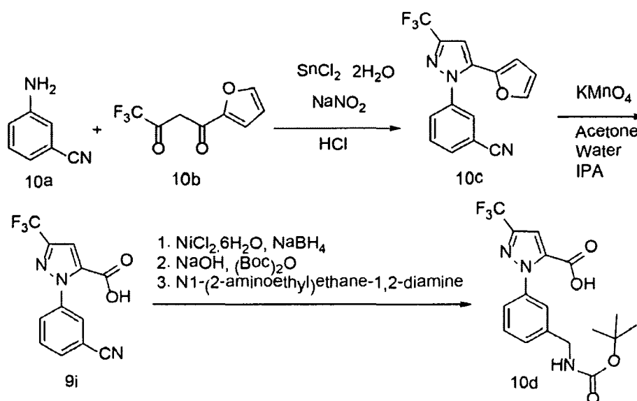
Scheme 10
