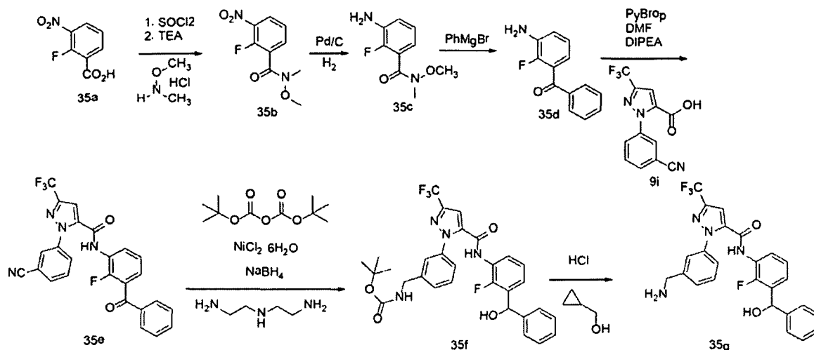
Scheme 35
