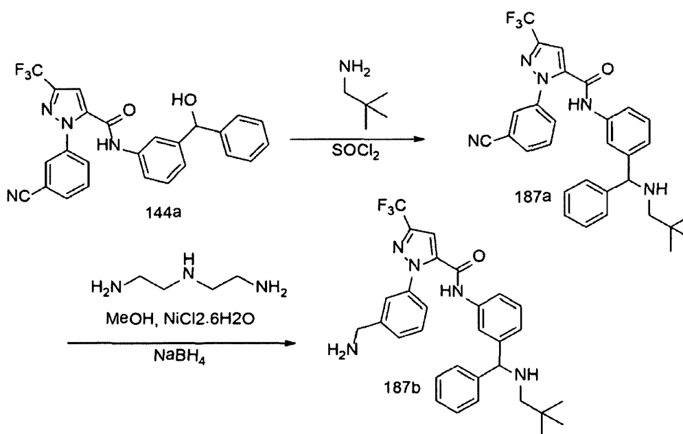
Scheme 187
