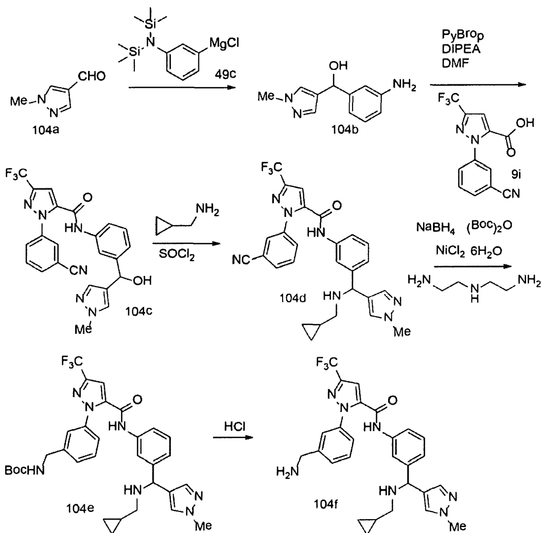
Scheme 104
