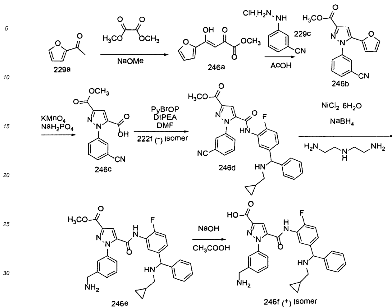
Scheme 246
