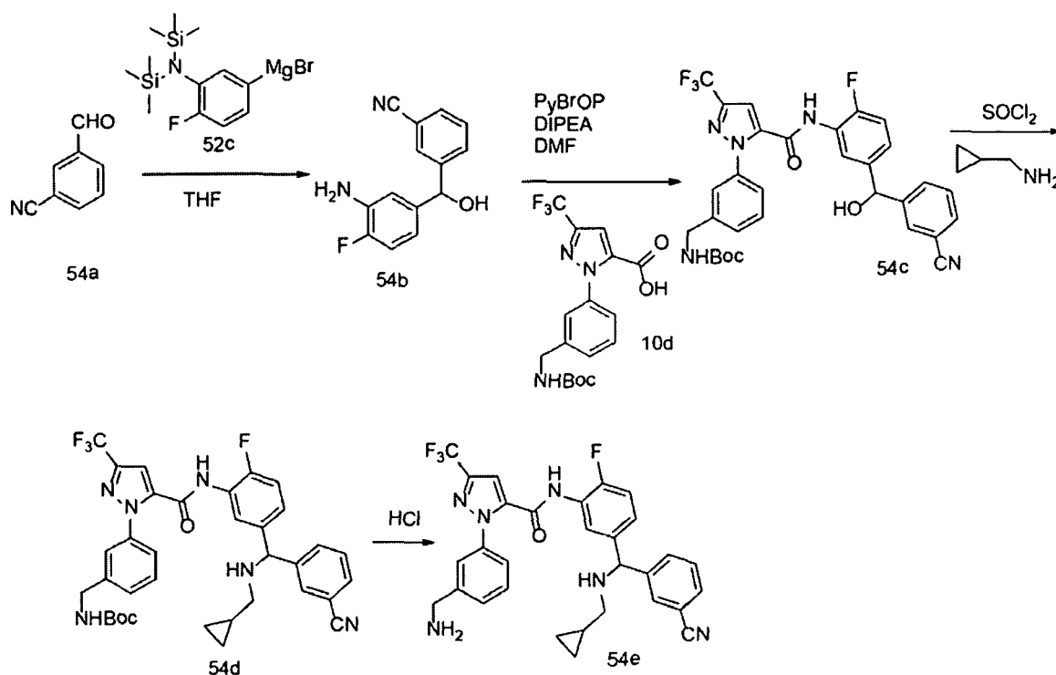
Scheme 54
