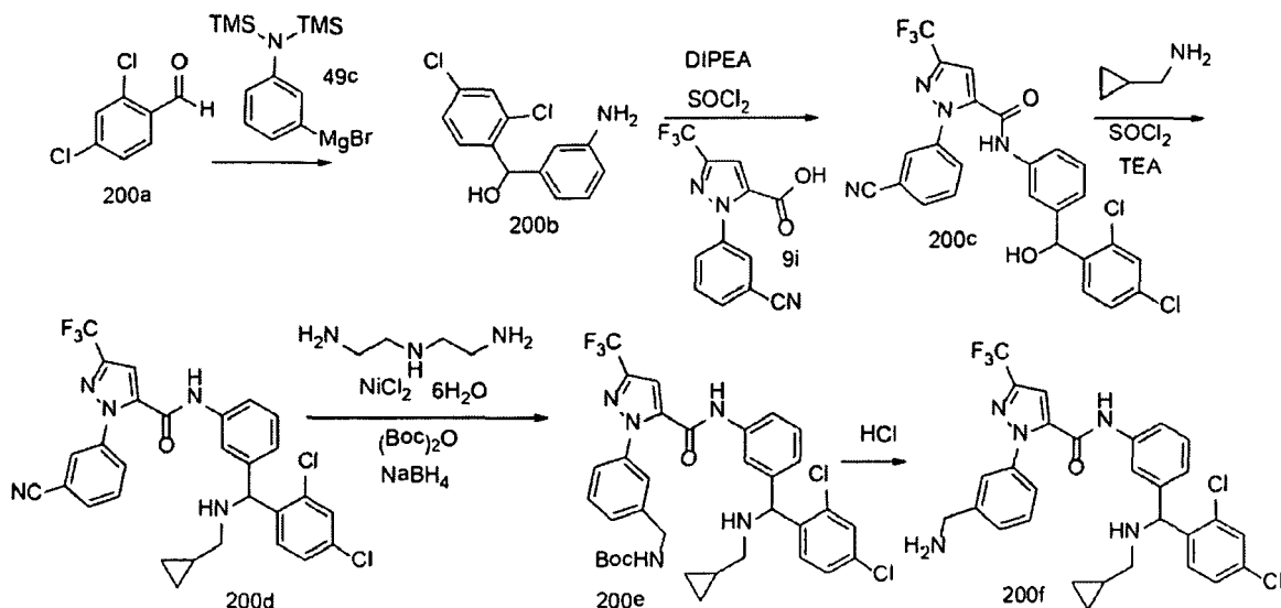
Scheme 200
