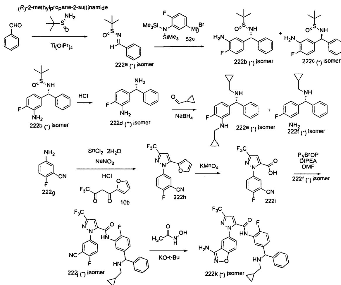
Scheme 222
