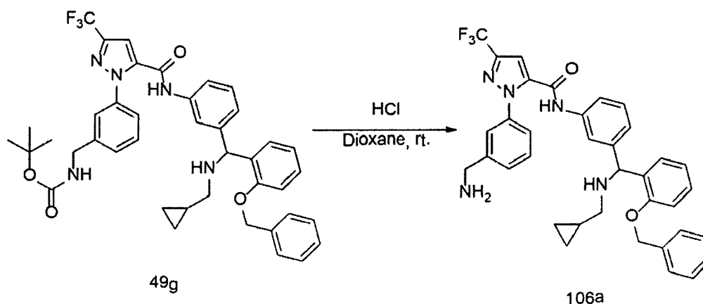
Scheme 106
