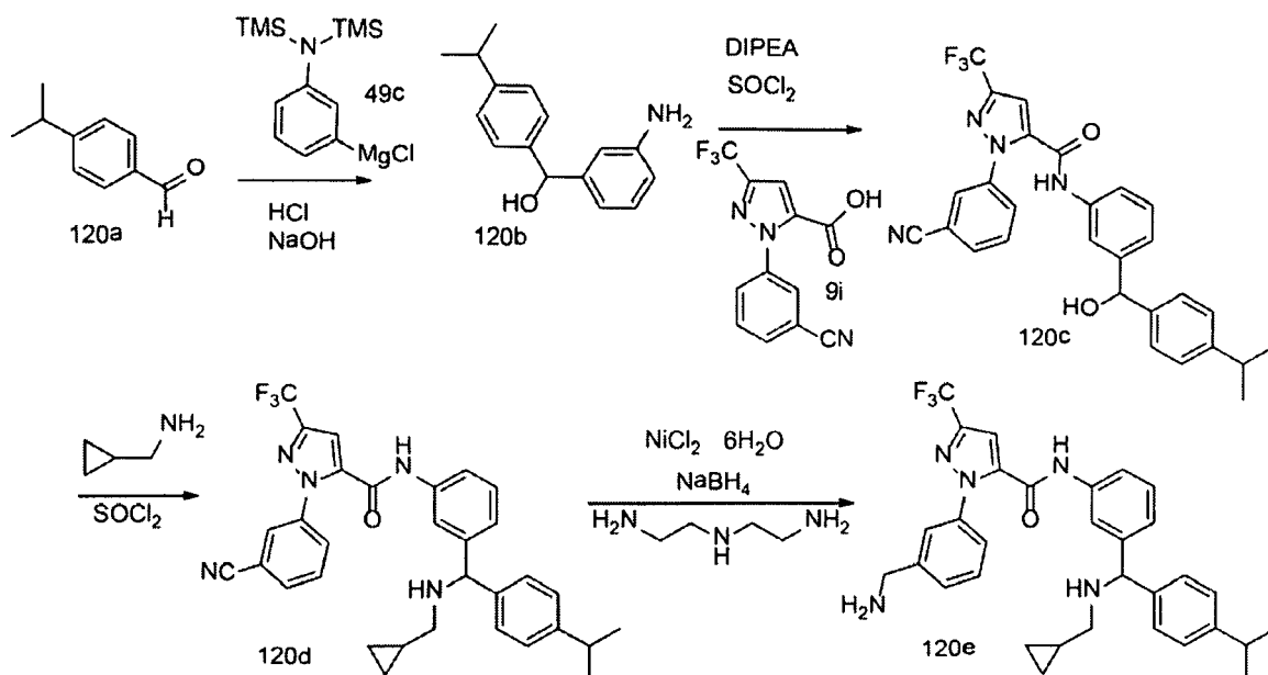
Scheme 120
