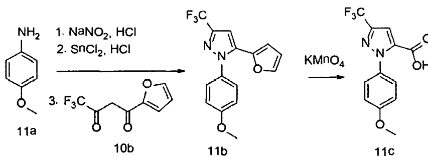
Scheme 11
