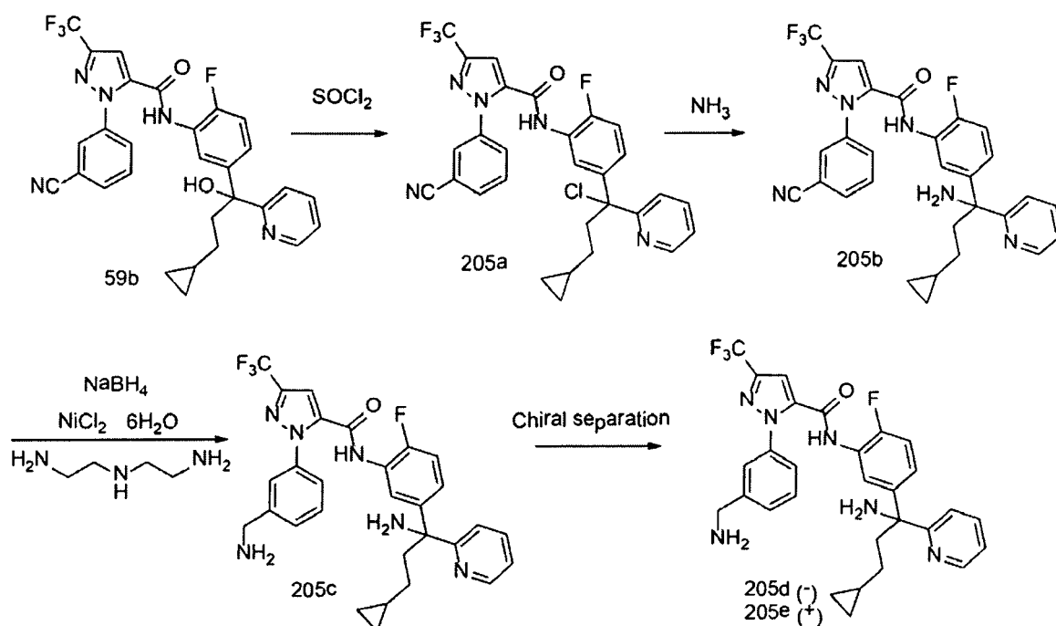
Scheme 205
