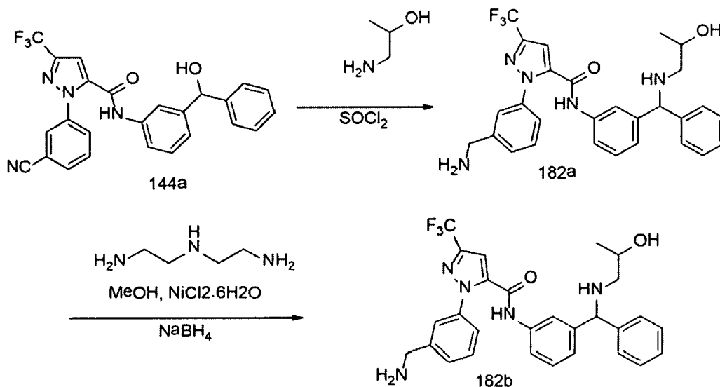
Scheme 182
