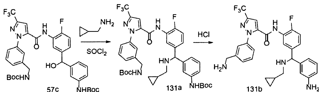
Scheme 131
