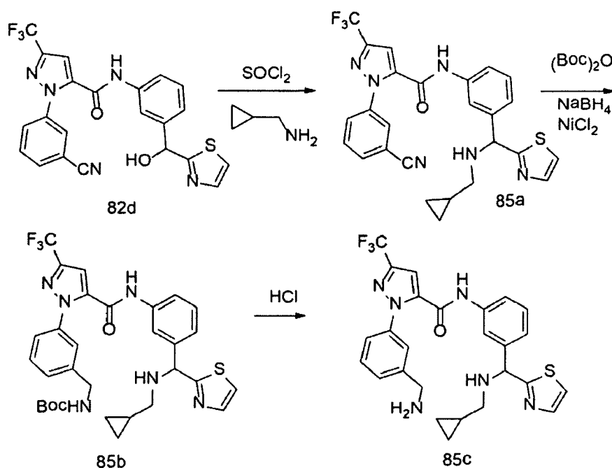
Scheme 85
