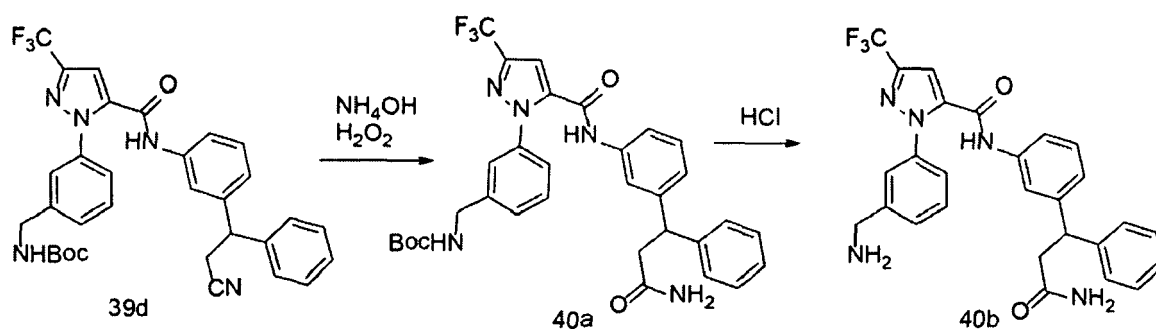
Scheme 40
