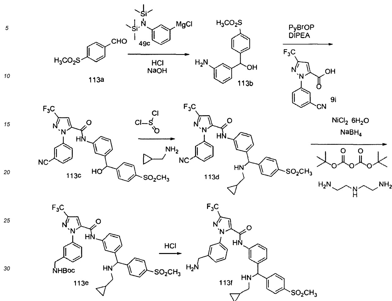
Scheme 113
