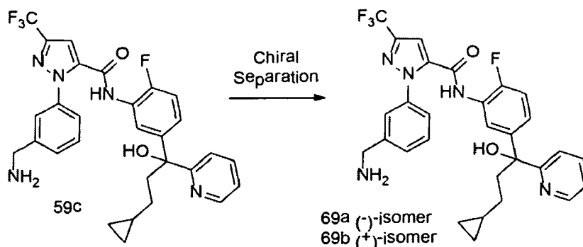
Scheme 69
