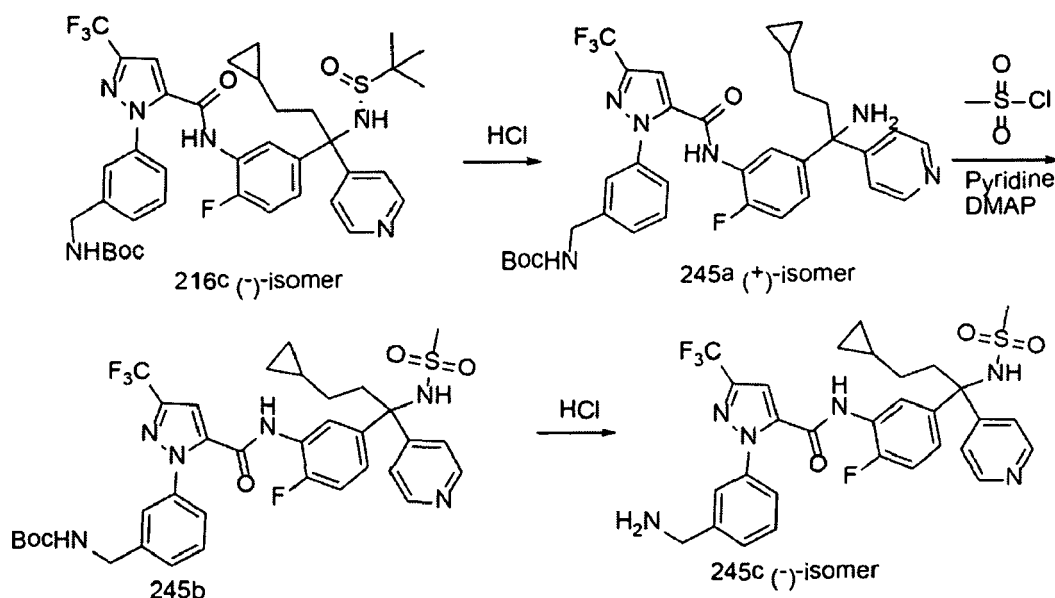
Scheme 245
