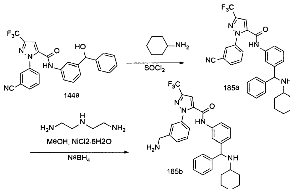
Scheme 185
