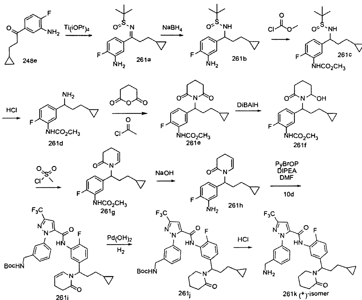
Scheme 261
