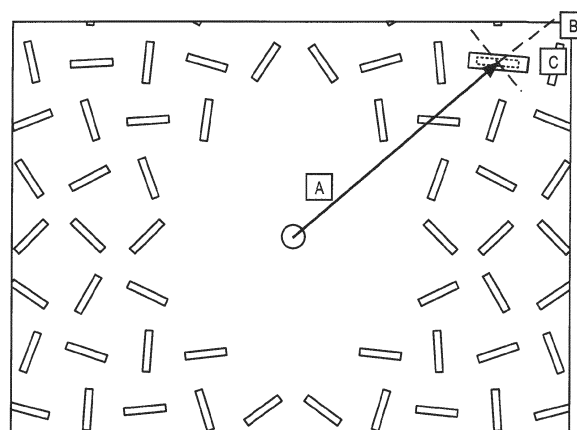
A = Solid black arrow denoting power feed vector from feed location to center of element B = Dashed orthogonal lines showing perpendicular axes relative to "A" C = Dashed rectangle encircling slot rotated 45 degrees relative to "B"
