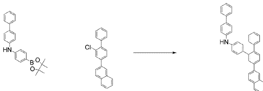
[Chem. 18]
