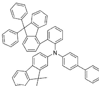
(HTM-3)
