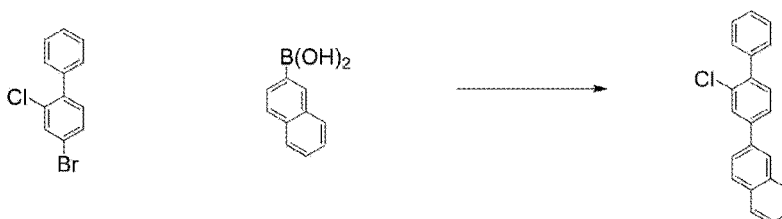
[Chem. 17]
