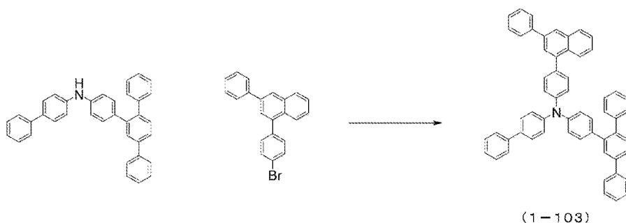
[Chem. 21]
