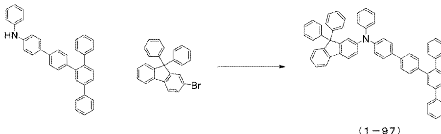
[Chem. 16]
