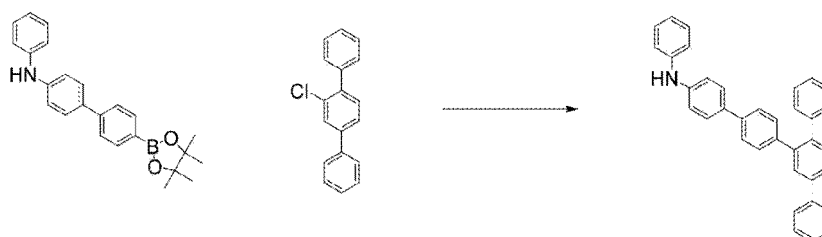
[Chem. 15]
