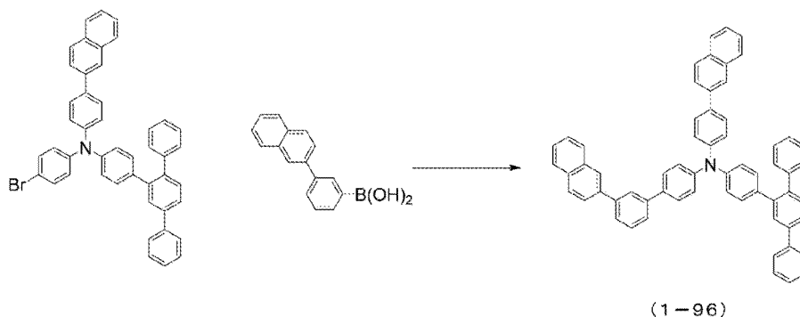
[Chem. 14]
