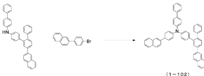
[Chem. 19]
