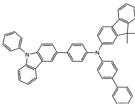
(HTM-2)
