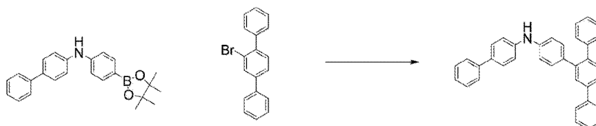
[Chem. 20]
