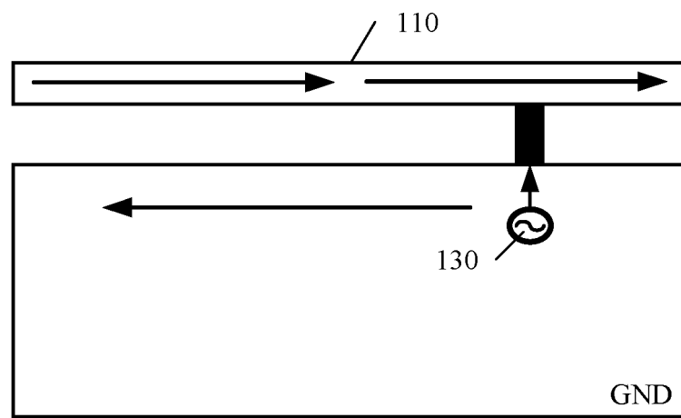
Current distribution in a third resonance
