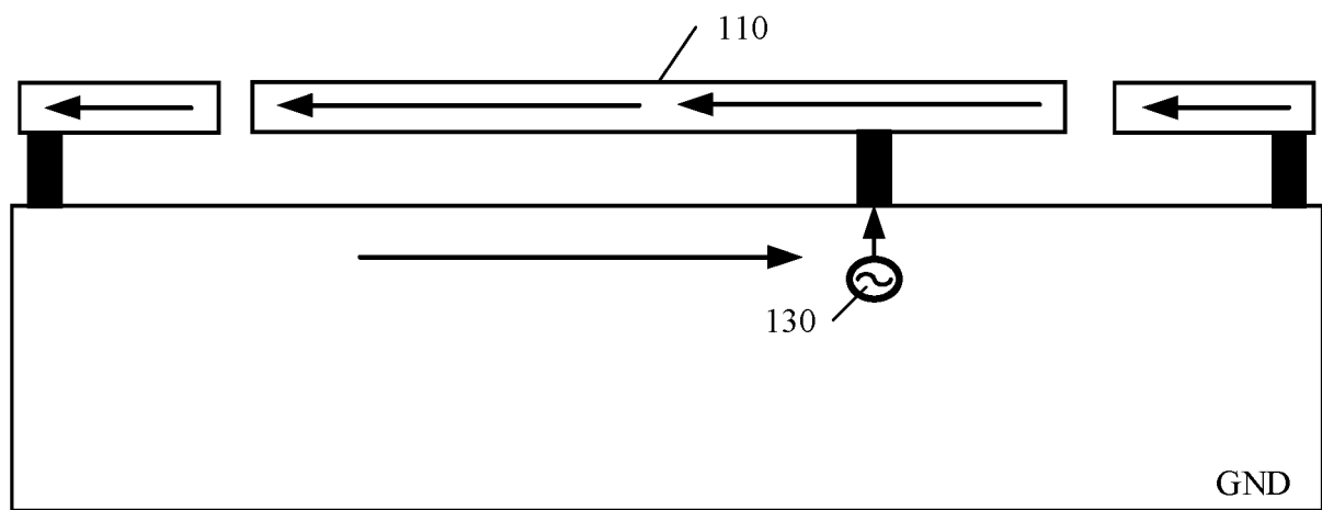
Current distribution in a third resonance
