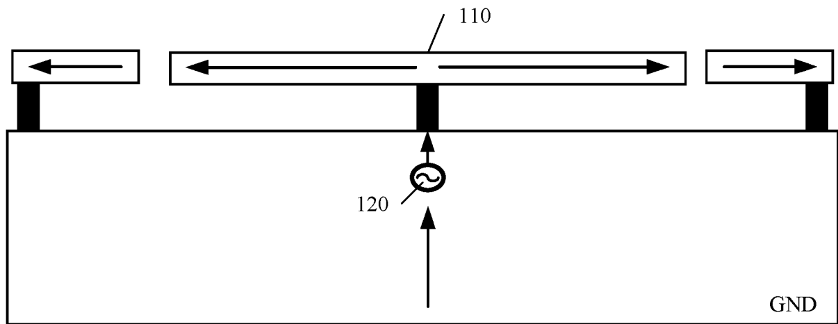
Current distribution in a first resonance
