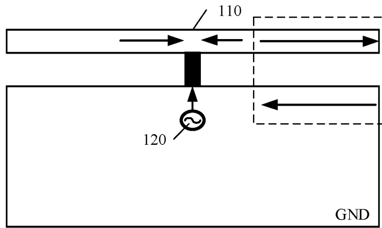
Current distribution in a second resonance
