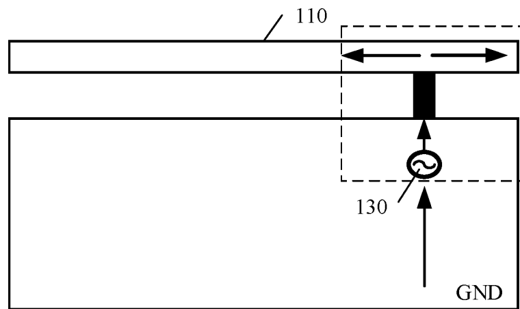
Current distribution in a fourth resonance
