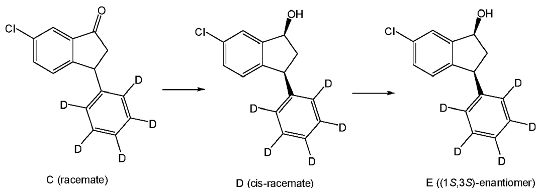
Scheme 2. Exemplary synthesis of intermediate E.
