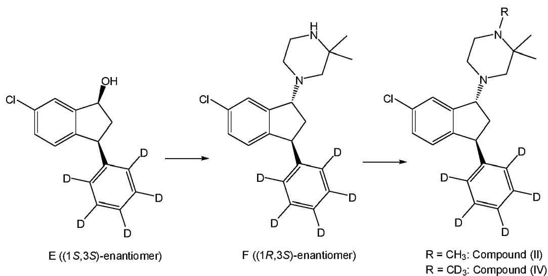
Scheme 5. Exemplary synthesis of intermediates F and Compounds (II) and (IV).
