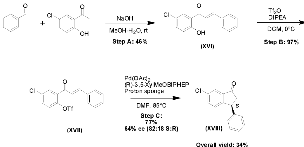
Scheme 15. Synthesis of Compound (XVIII)
