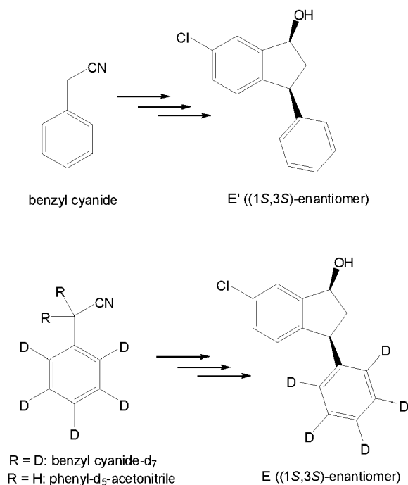
Scheme 4. Exemplary synthesis of intermediates E and E'.
