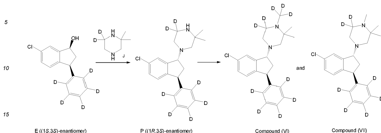
Scheme 13. Synthesis of Compound (VI) and Compound (VII).
