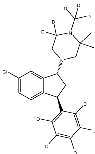
(1R,3S)-(VI).
