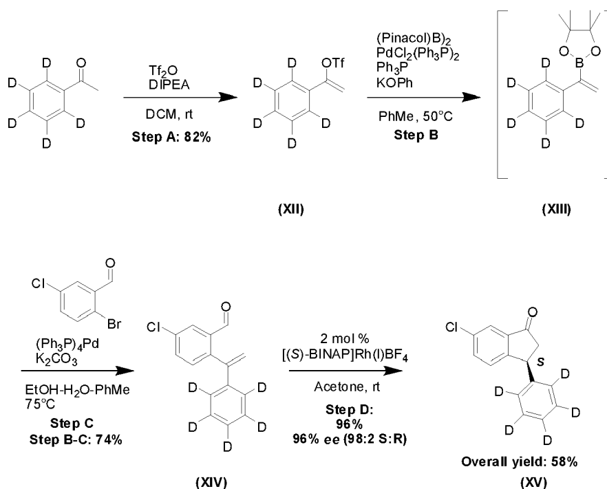
Scheme 14. Synthesis of Compound (XV)
