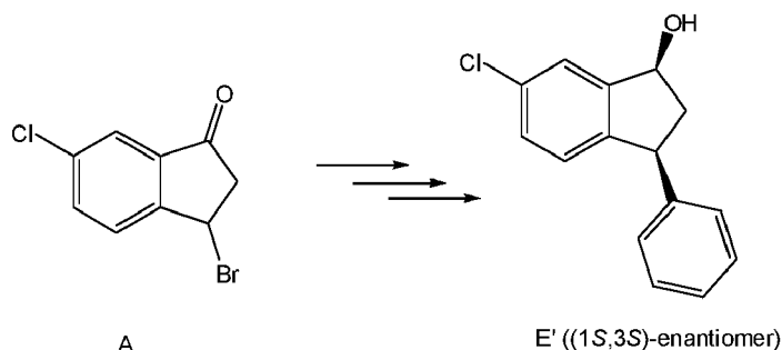
Scheme 3. Exemplary synthesis of intermediate E'.
