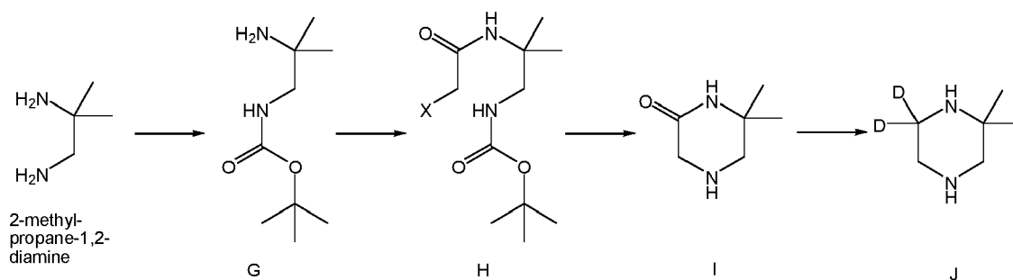
Scheme 6. Exemplary synthesis of intermediate J.
