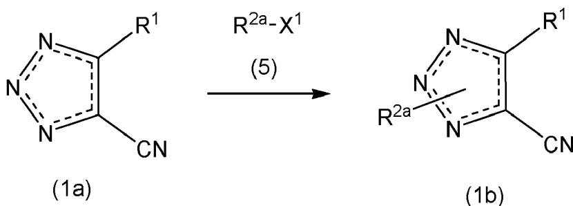
Reaction Scheme 2
