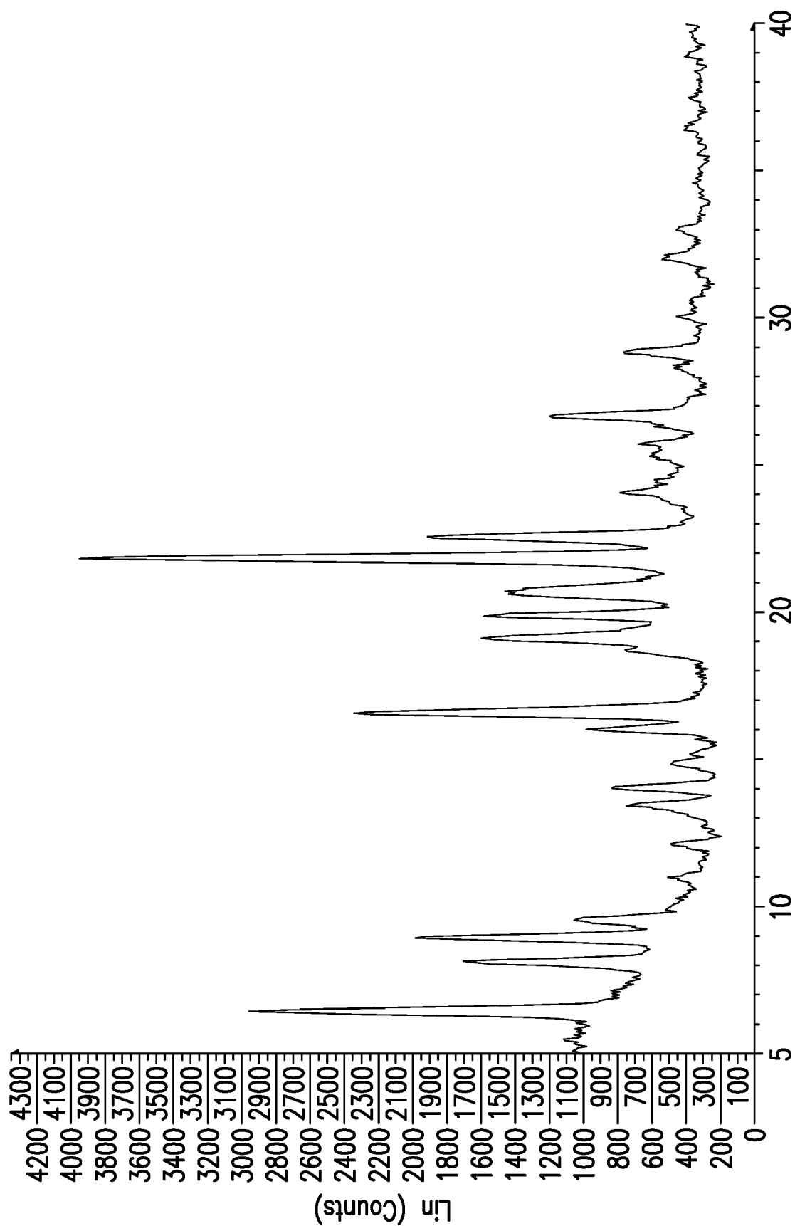
2-Theta - Scale
