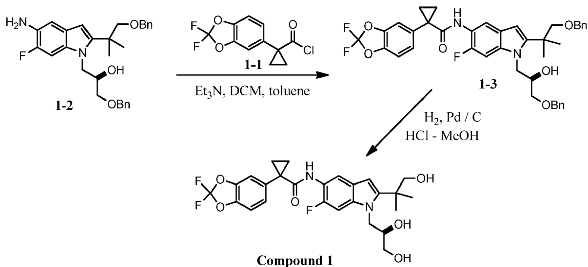
Scheme 1: Preparation of Compound 1.
