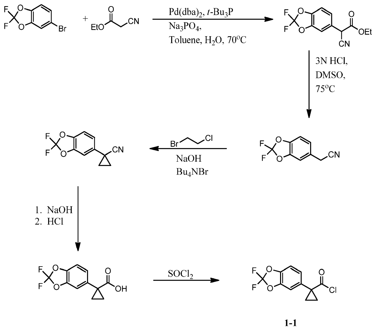
Scheme 2: Preparation of Compound 1-1.
