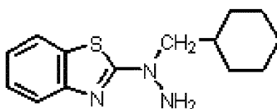
Intermediate S
