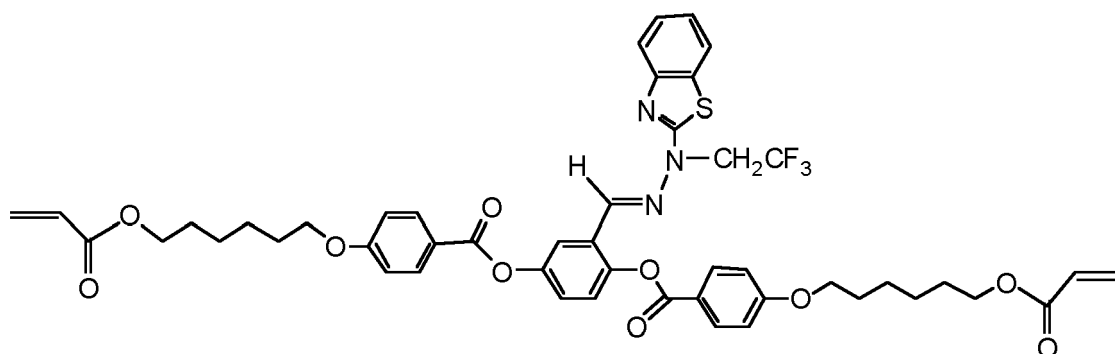
Compound 13
