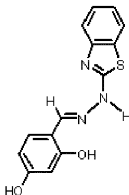
Intermediate Q
