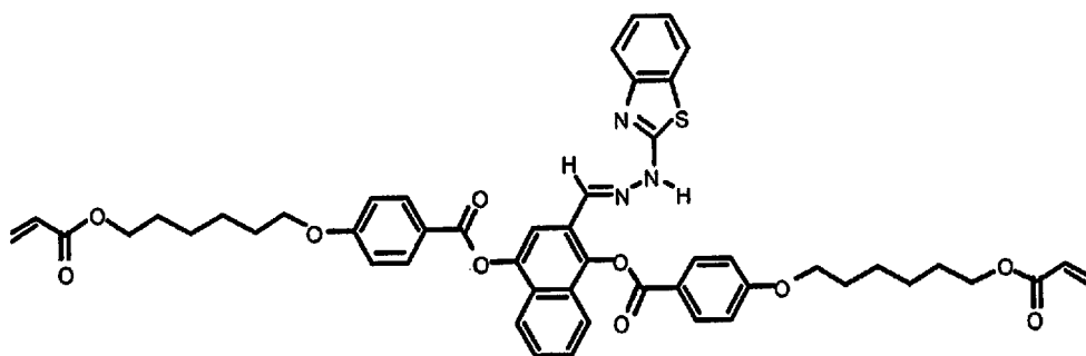
Compound 22
