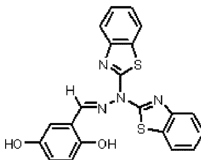
Intermediate K
