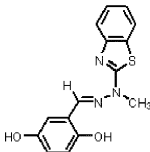
Intermediate E
