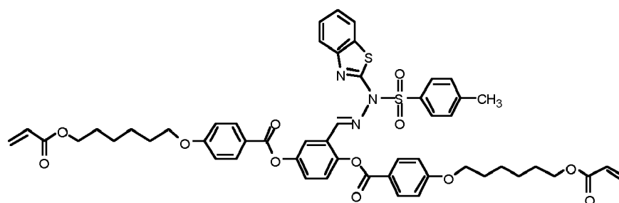
Compound 27
