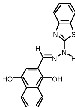
Intermediate c
