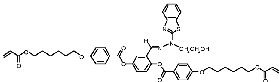
Compound 32
