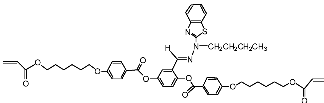
Compound 8
