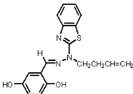
Intermediate X
