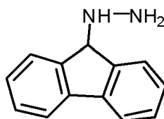
Intermediate m
