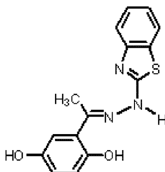
Intermediate P
