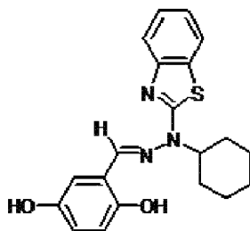
Intermediate i
