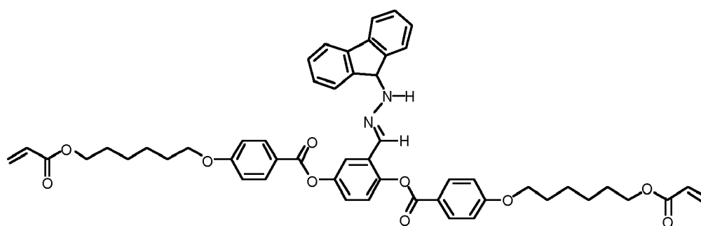
Compound 33
