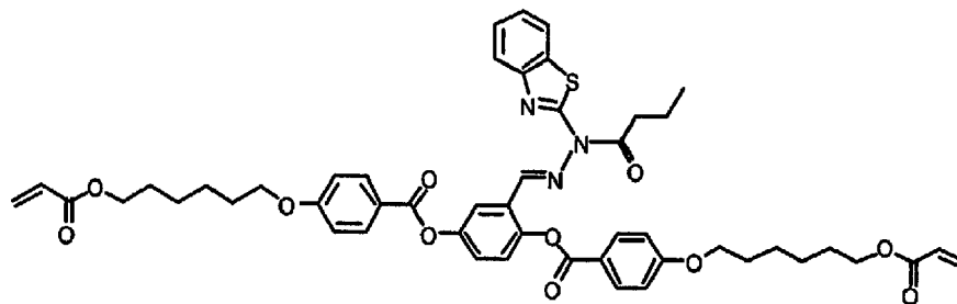
Compound 29
