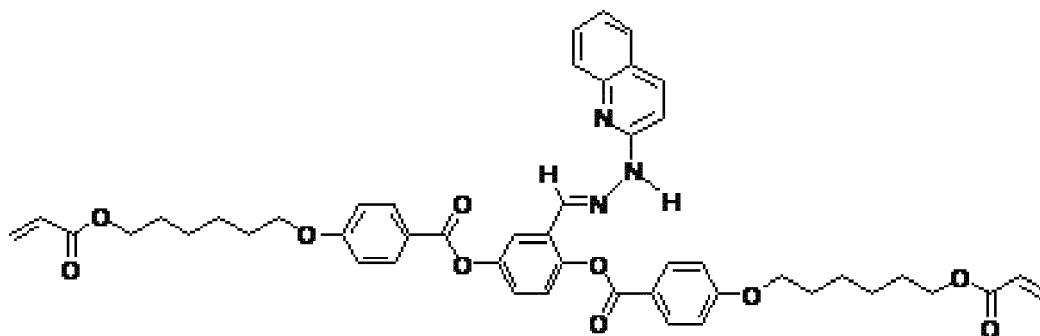
Compound 5
