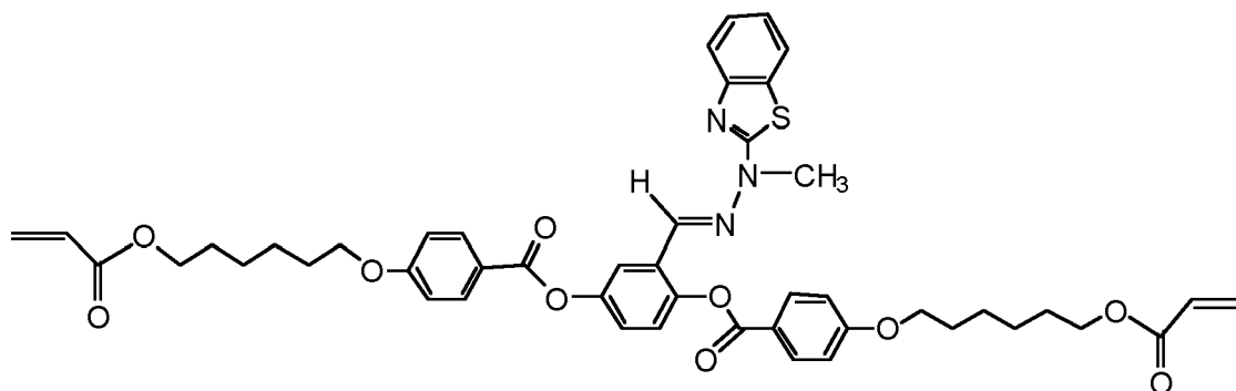
Compound 7
