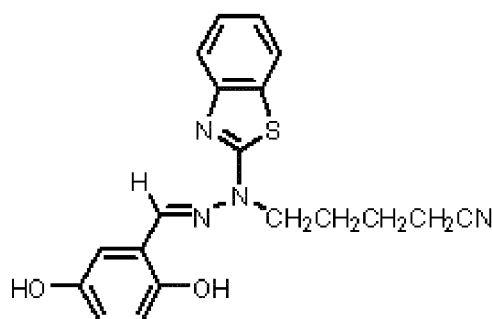
Intermediate V
