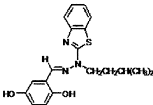
Intermediate k
