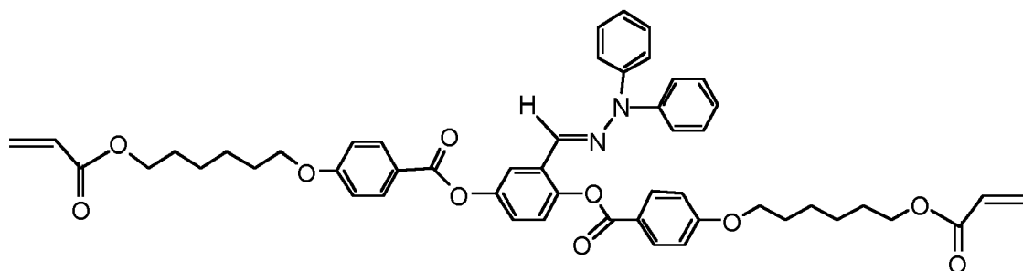
Compound 4
