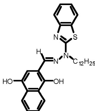
Intermediate o
