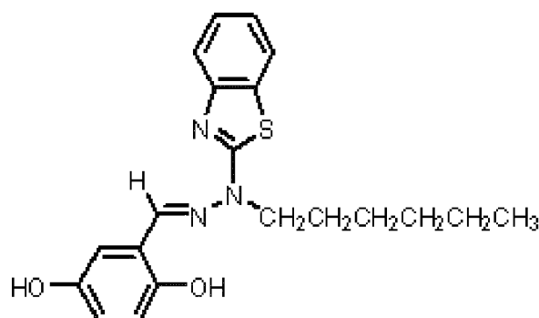
Intermediate I
