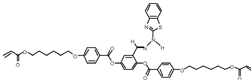
Compound 1
