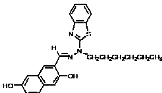
Intermediate f
