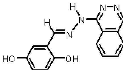
Intermediate C
