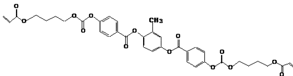
Compound 2r
