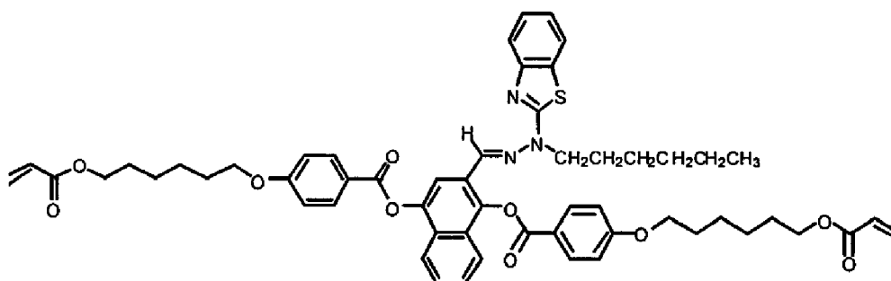
Compound 24
