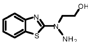
Intermediate 1
