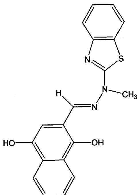
Intermediate d
