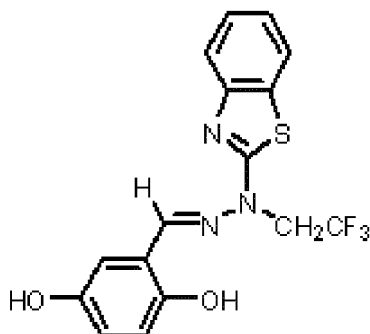
Intermediate O
