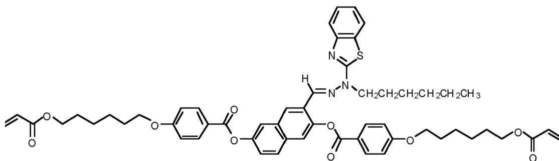
Compound 25
