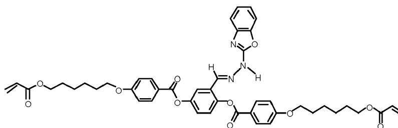
Compound 2
