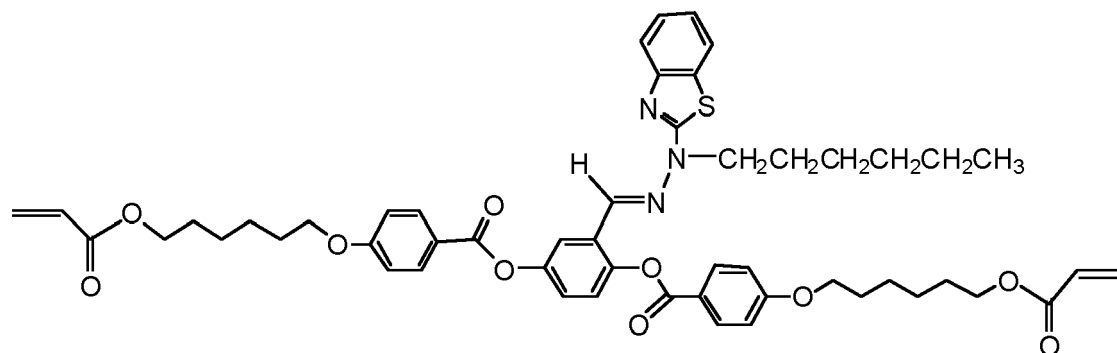
Compound 9
