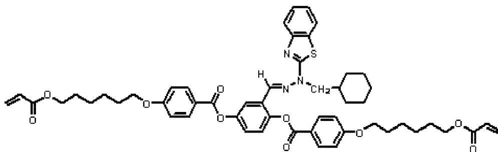
Compound 17
