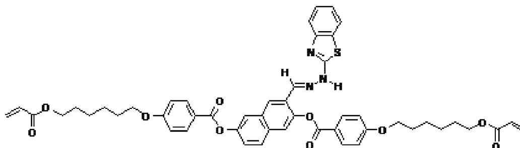
Compound 26
