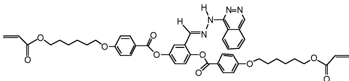
Compound 6
