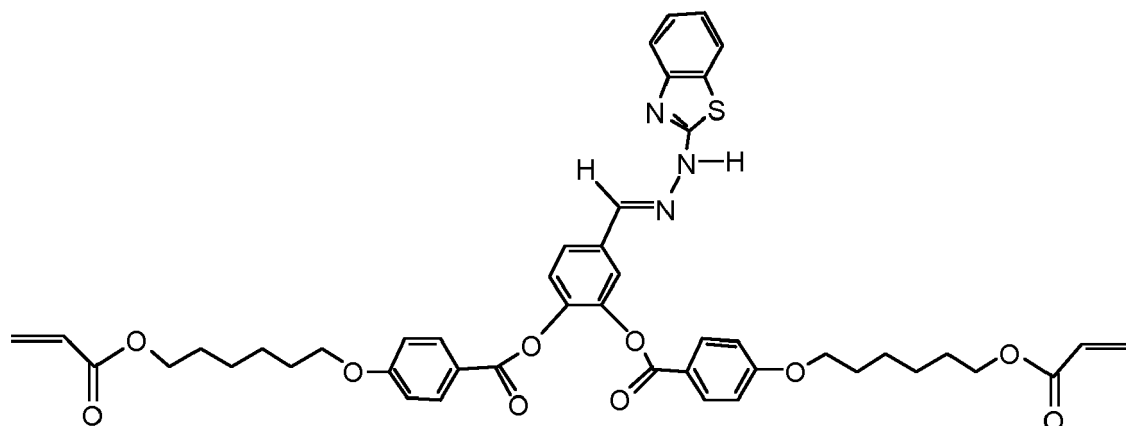
Compound 16
