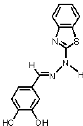
Intermediate R
