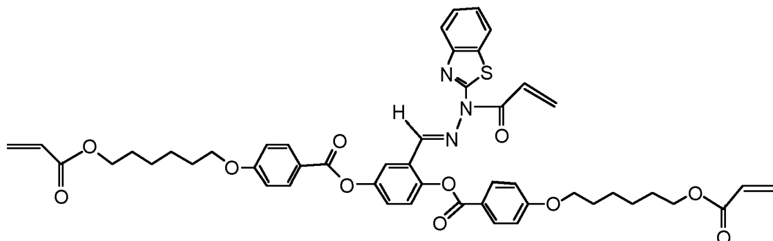
Compound 10
