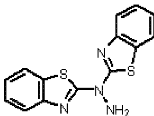
Intermediate J
