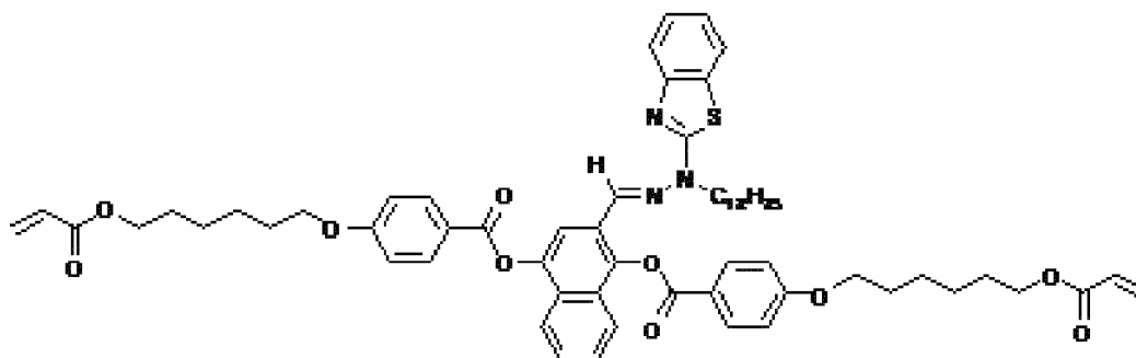
Compound 34
