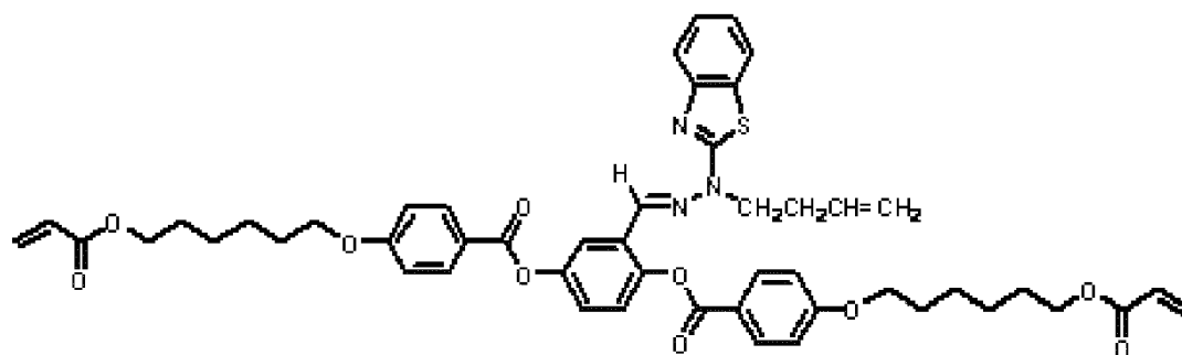
Compound 19
