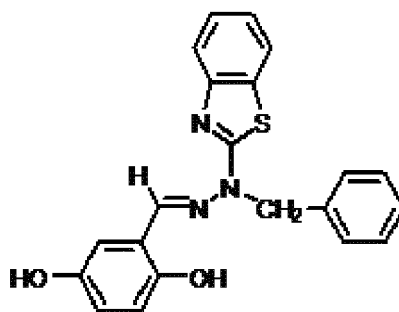
Intermediate b
