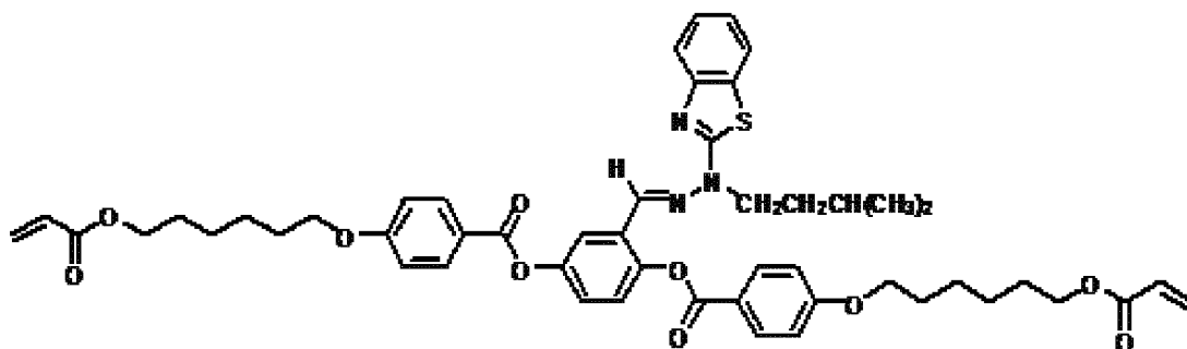
Compound 31
