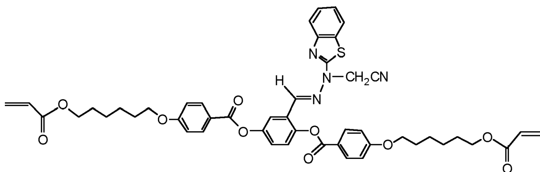
Compound 12
