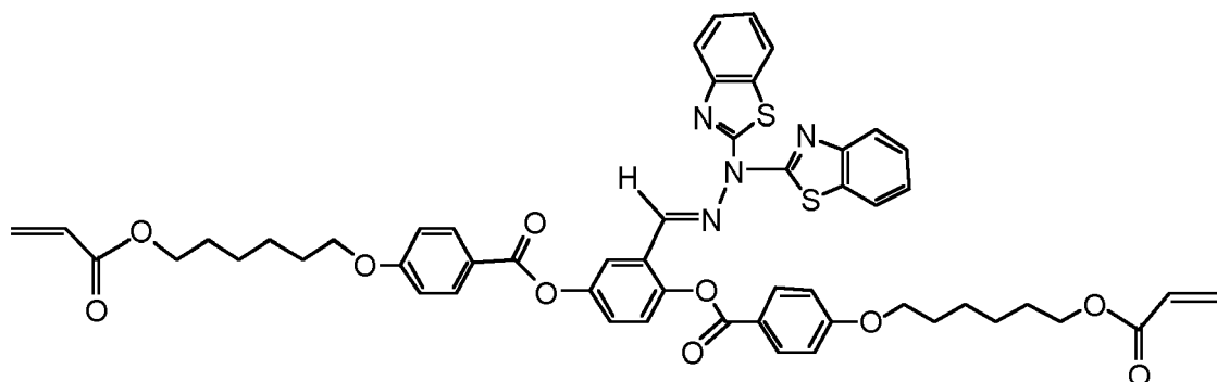
Compound 11
