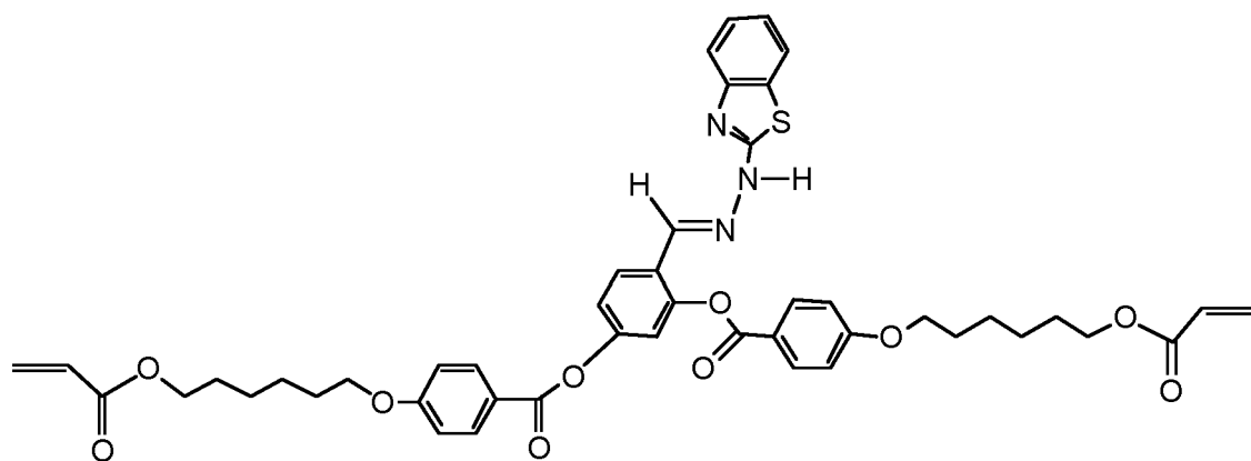
Compound 15
