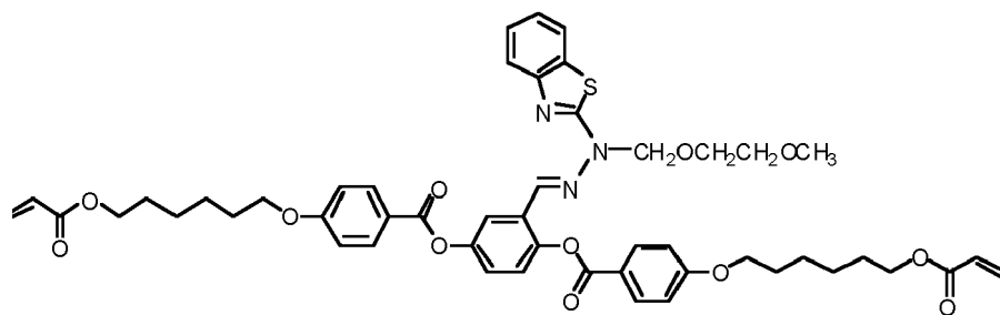
Compound 28
