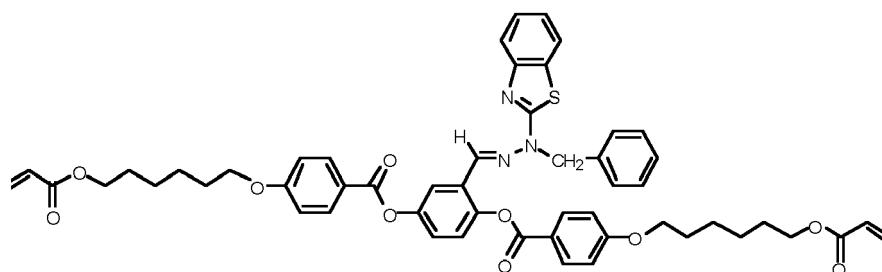
Compound 21
