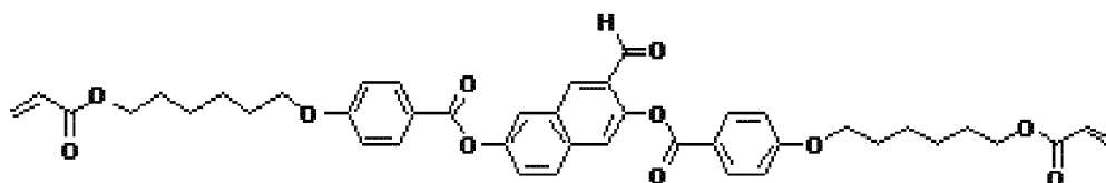
Intermediate g
