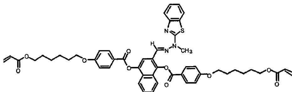
Compound 23
