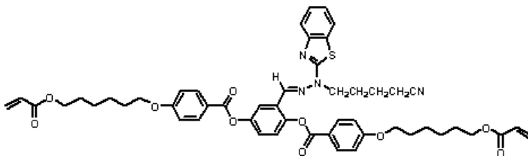
Compound 18
