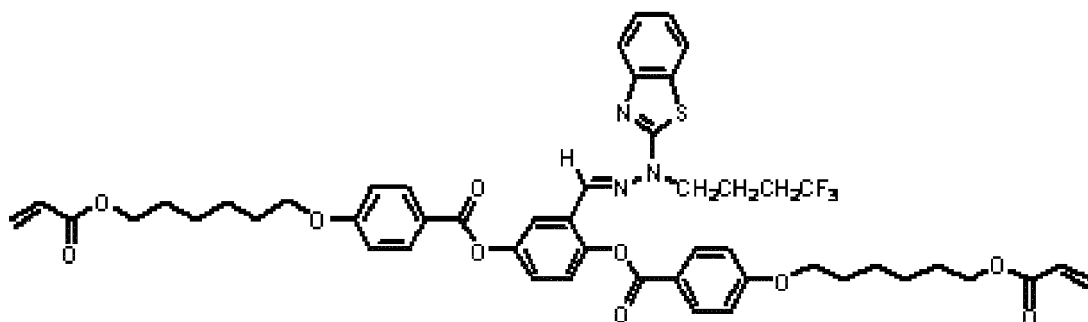
Compound 20
