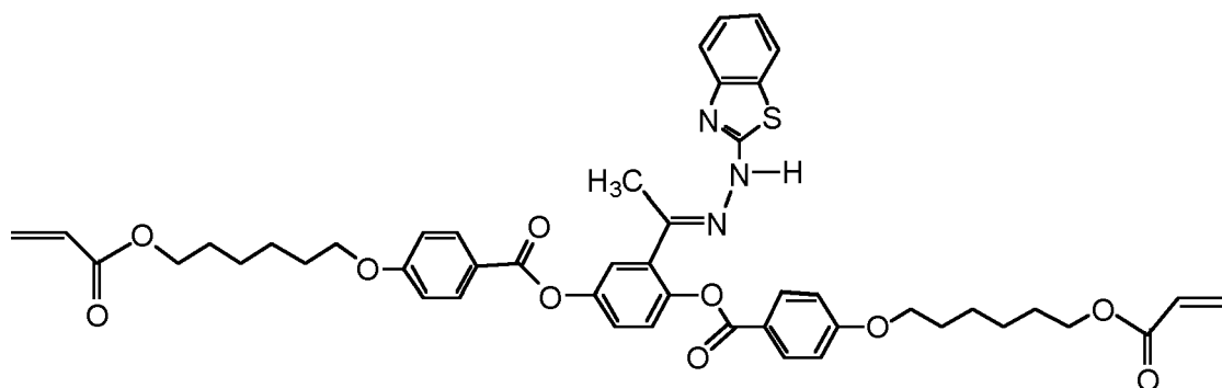
Compound 14
