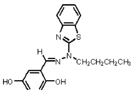
Intermediate G
