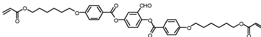
Intermediate A
