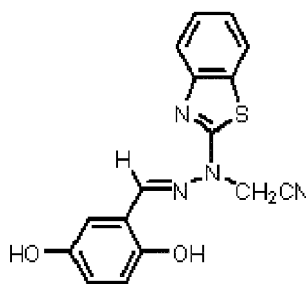
Intermediate M
